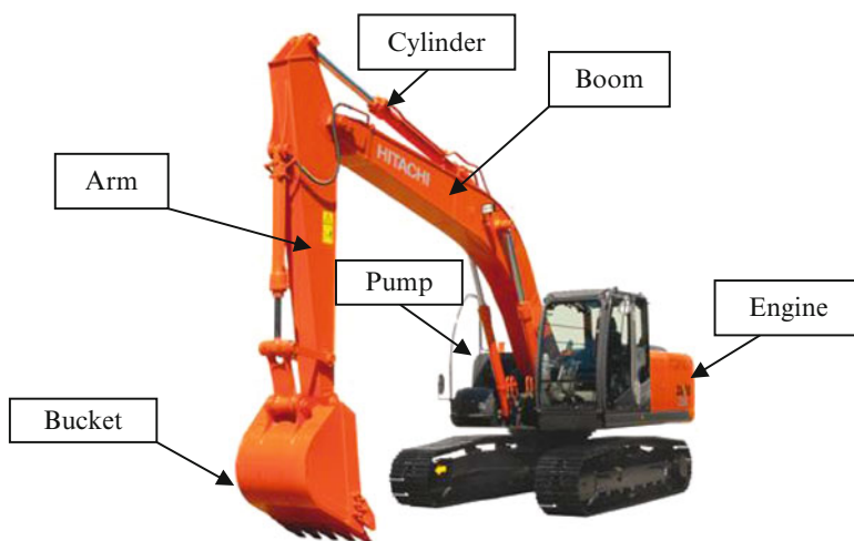
Fig. 8.1 Hydraulic excavator
