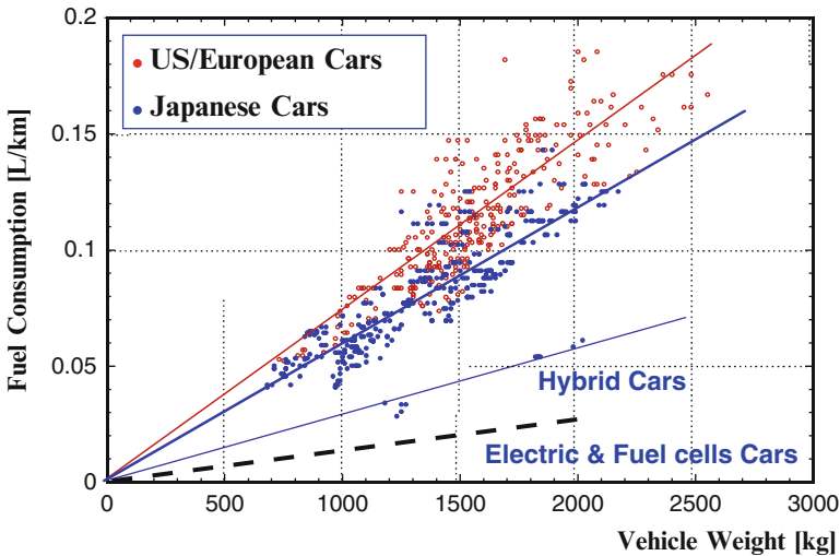
Fig. 3.1 Automobile energy consumption to 1/10 at 2050. (Data from Yahoo! Jidosha)
