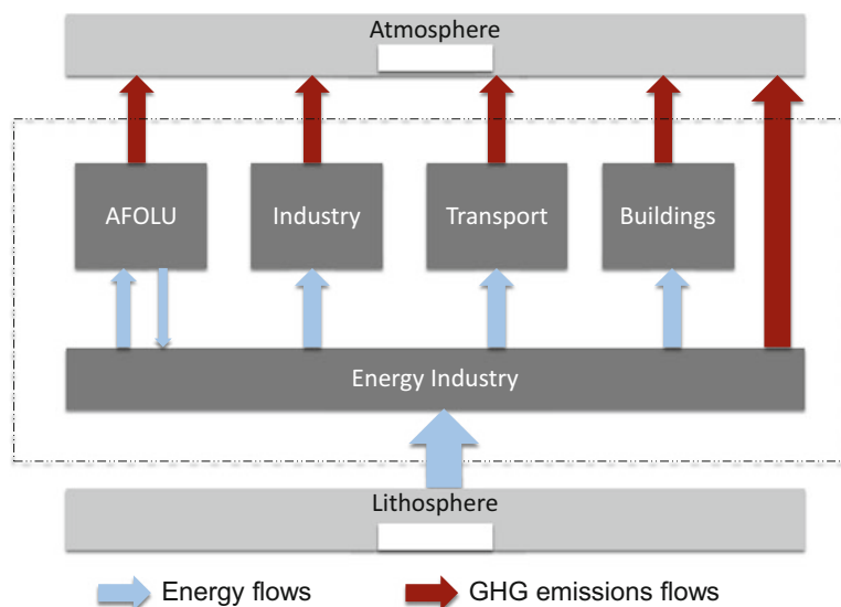
Fig. 6.1 Summary of the standard approach for emissions accounting, e.g. 2006 IPCC Guidelines for National Greenhouse Gas Inventories (IPCC 2006)
