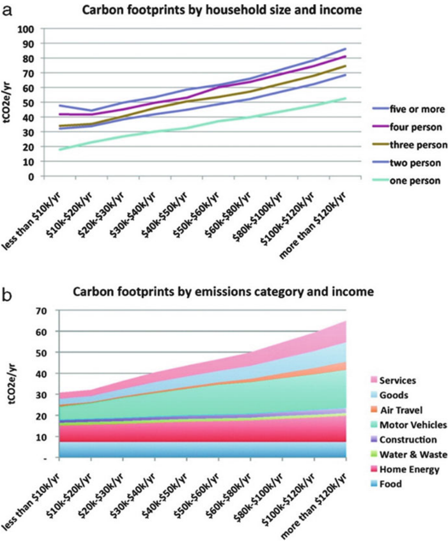
Fig. 9.2 (a) Carbon footprints by income bracket and household size; (b) Carbon footprints by category of emissions and income bracket for average household size of 2.5 persons (Source: Jones and Kammen (2011), Fig. 2, p. 4090)
