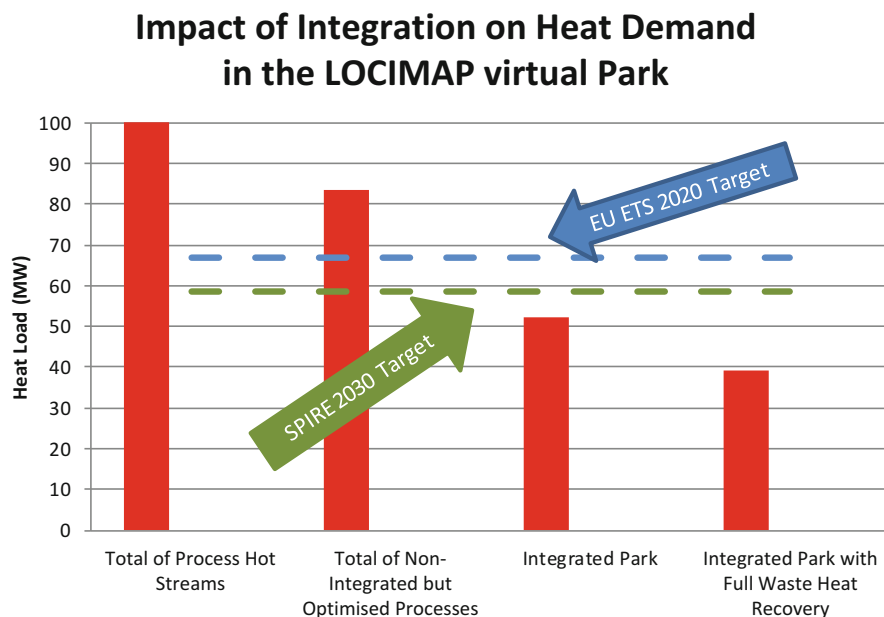
Fig. 19.3 Impact of process integration within a virtual ‘LOCIMAP’ park
