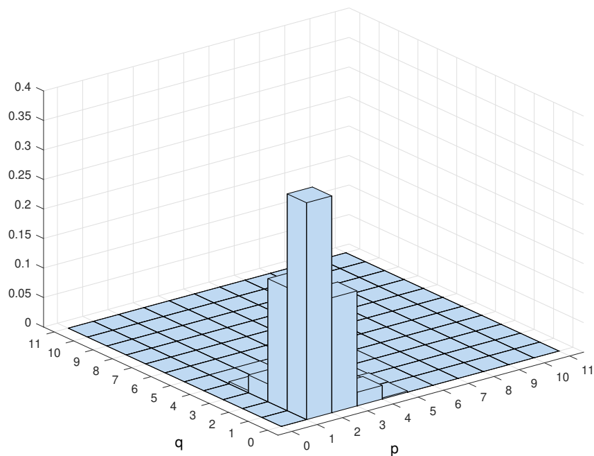
Figure 5: Posterior over the orders for the shock process, synthetic AR(1) data from (18)
