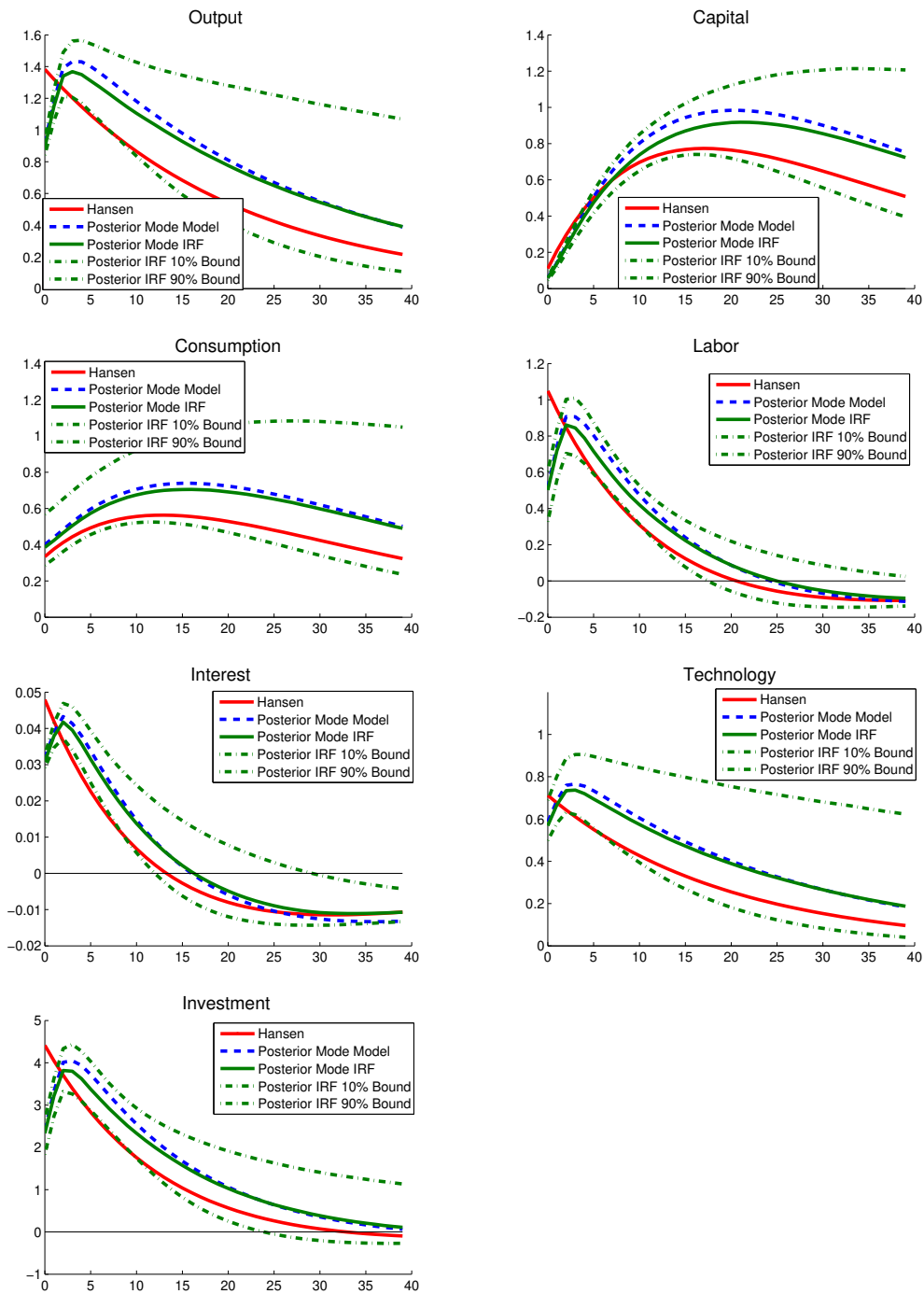
Figure 10: Impulse responses to a one standard deviation technology shock Invertibility of MA components imposed HP filtered data and model along with Hansen's (1985) original AR(1) specification
