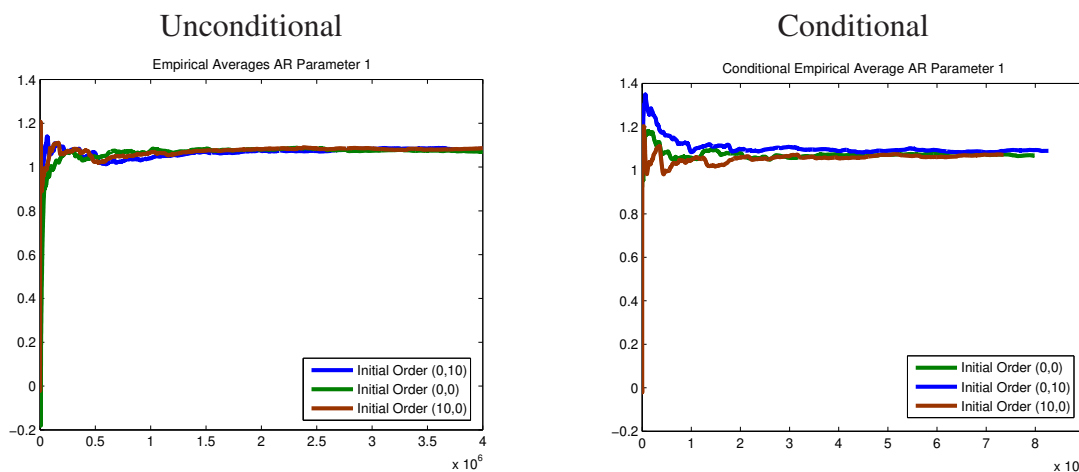
Figure 8: Convergence diagnostics, HP filtered data and model
