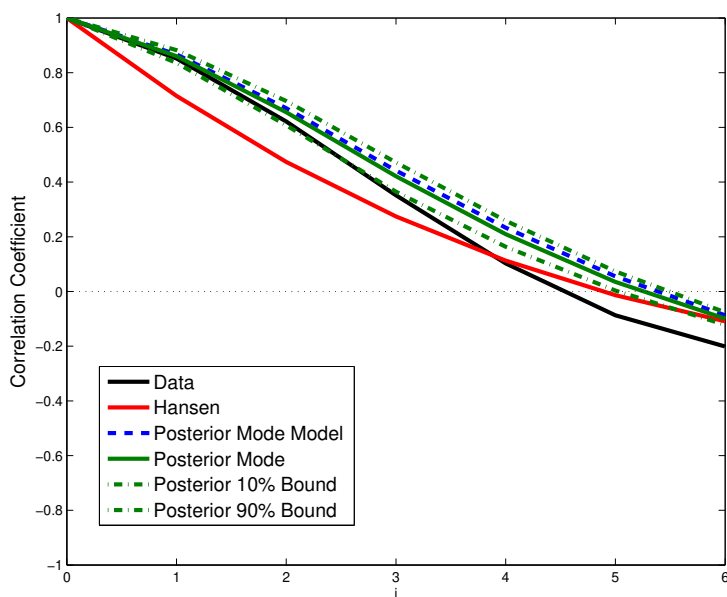
Figure 9: Comparison of autocorrelations of output, HP filtered data and model
