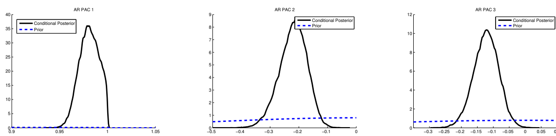
Figure 7: Priors and posteriors for partial autocorrelations, HP filtered data and model
