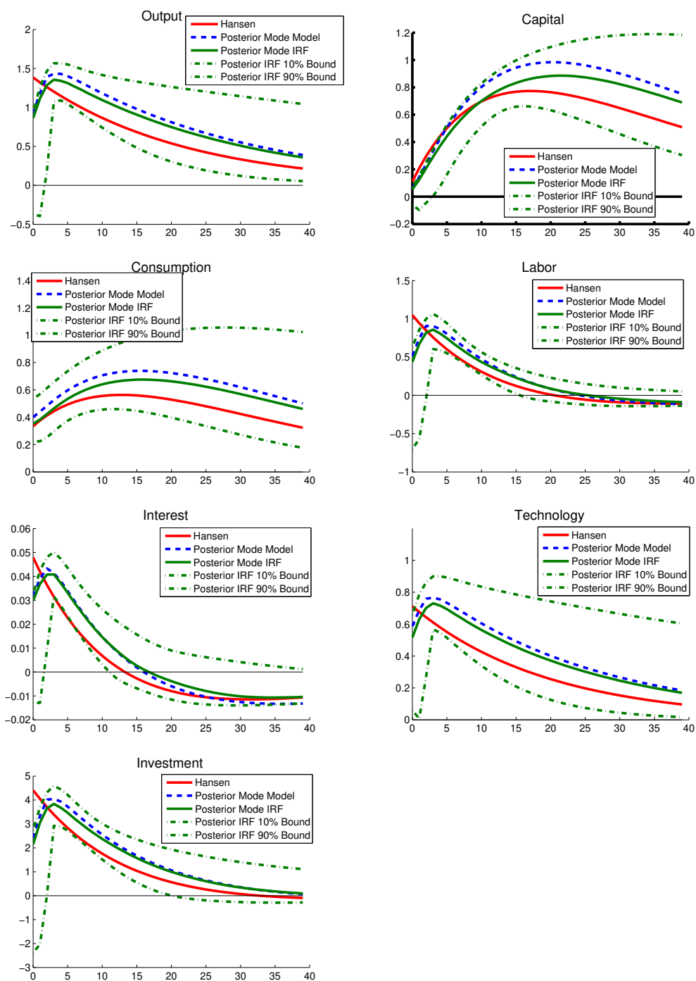
Figure 11: Impulse responses to a one standard deviation technology shock Invertibility of MA components not imposed HP filtered data and model along with Hansen's (1985) original AR(1) specification
