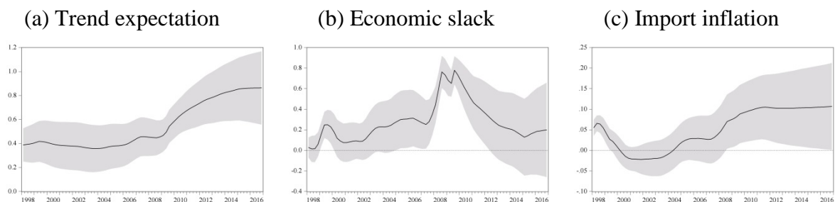
Figure 13: Time-varying Coefficient Estimates: Malaysia
