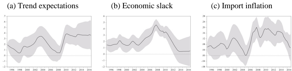
Figure 17: Time-varying Coefficient Estimates: Singapore
