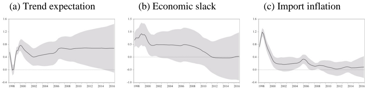
Figure 11: Time-varying Coefficient Estimates: Indonesia
