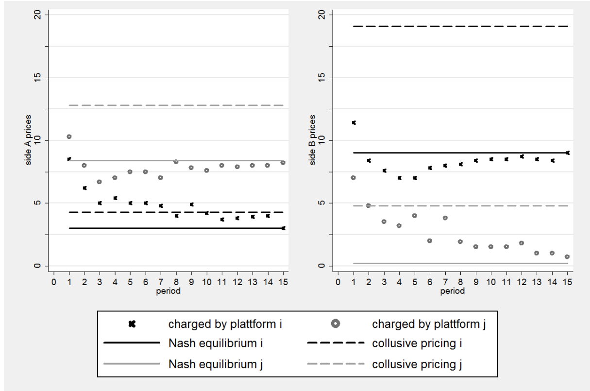
Figure 3: Median prices over periods in treatment d-asy .
