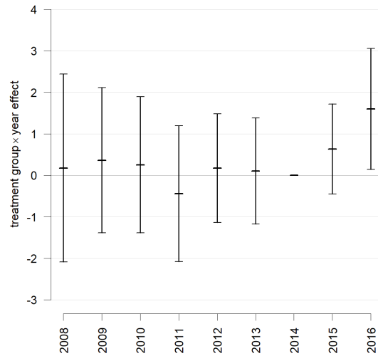
Figure 10: Event study design: demolitions of small residential buildings
