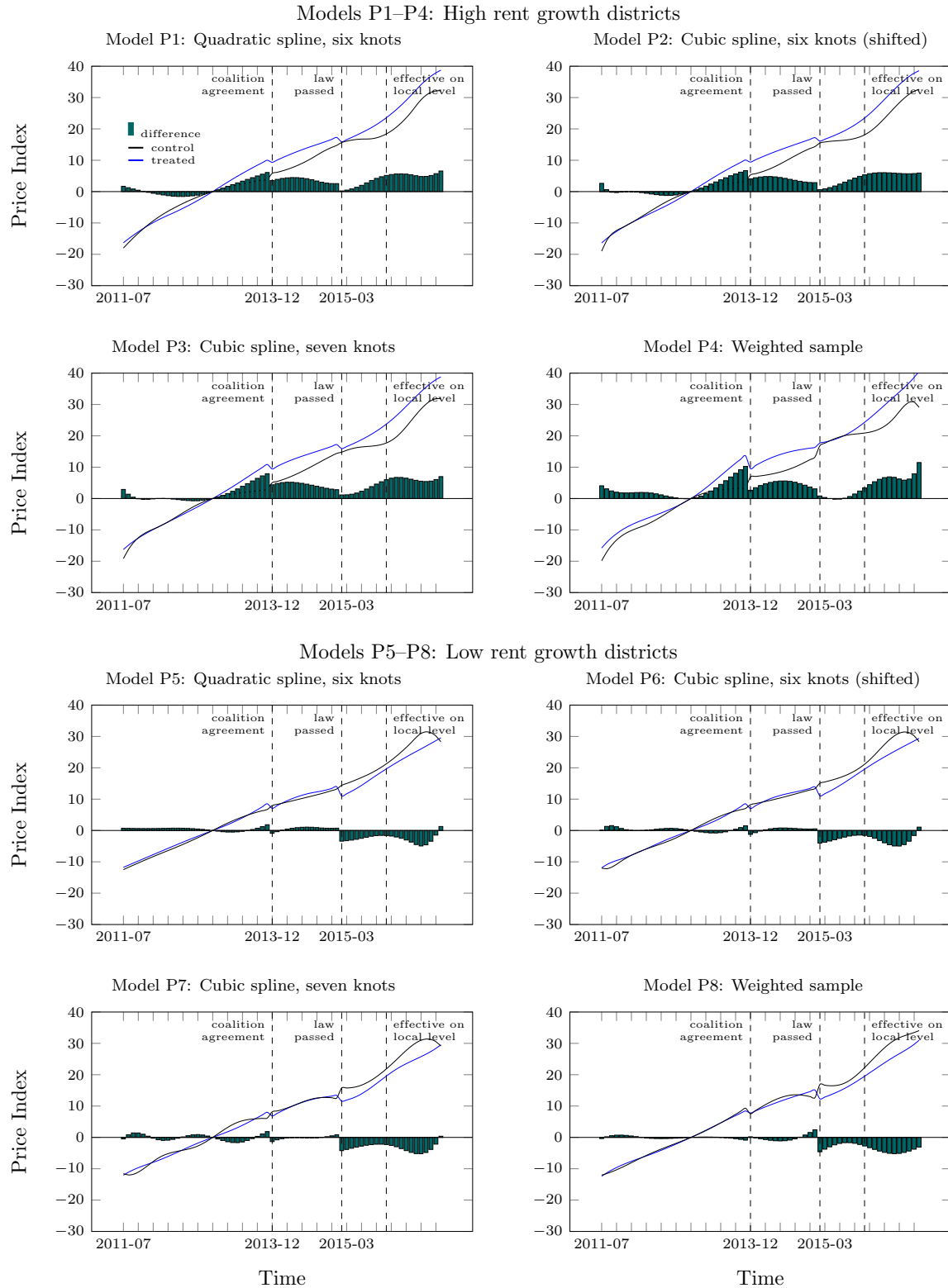
Figure 16: Robustness checks: effects of the rent cap on prices, see Table 15
