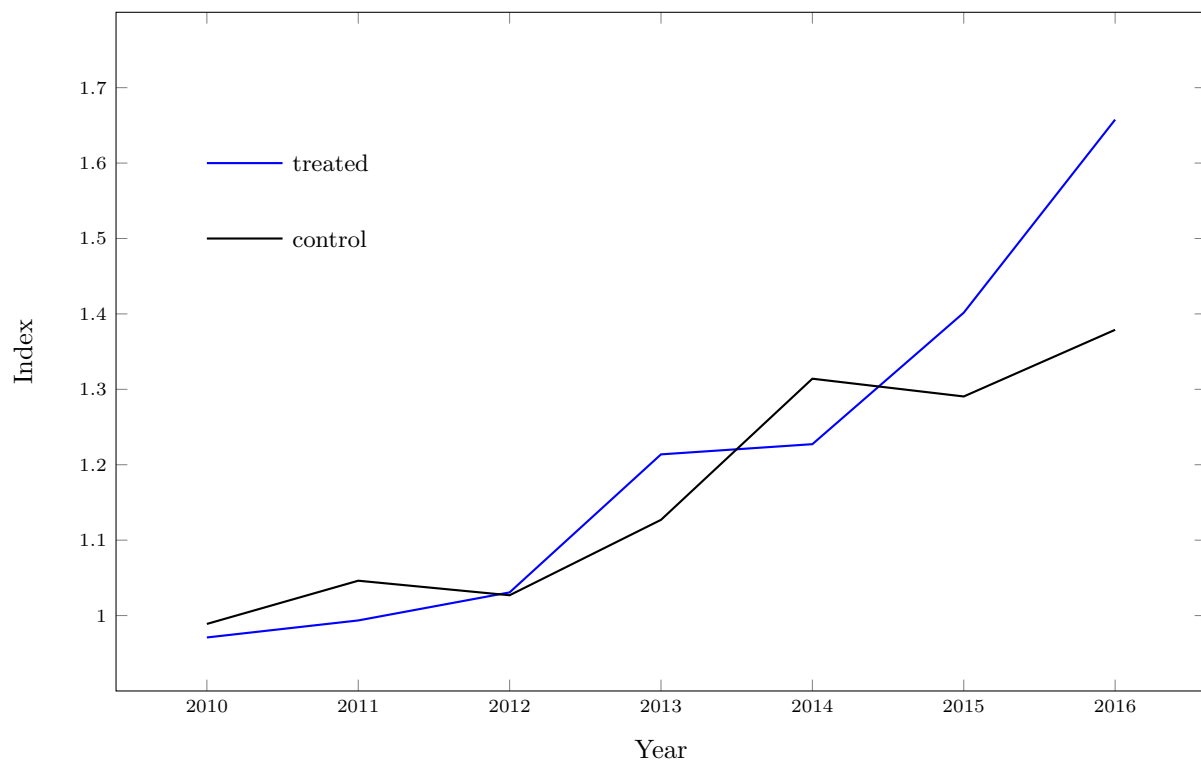
Figure 17: Land values in Bavaria: treatment and control groups in the trimmed and weighted sample
