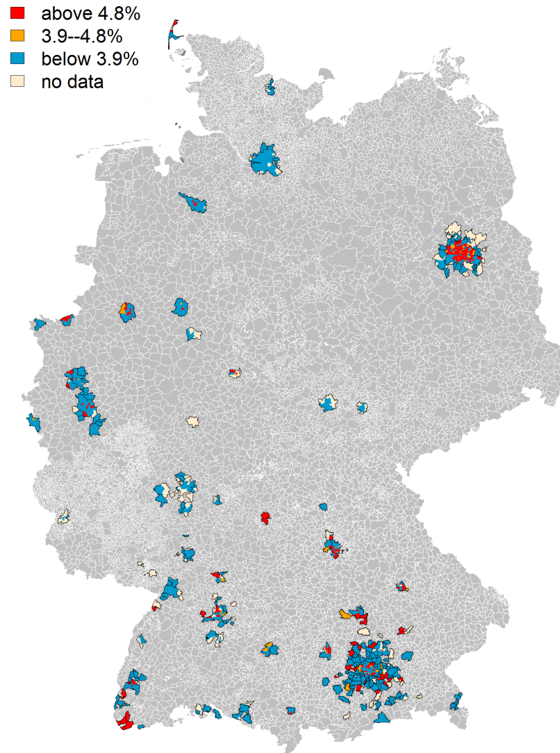
Figure 12: de facto regulated and unregulated postal code districts, as of June 2016
