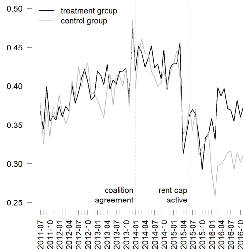
Figure 11: Share of units offered for sale, predicted to be a rental unit
