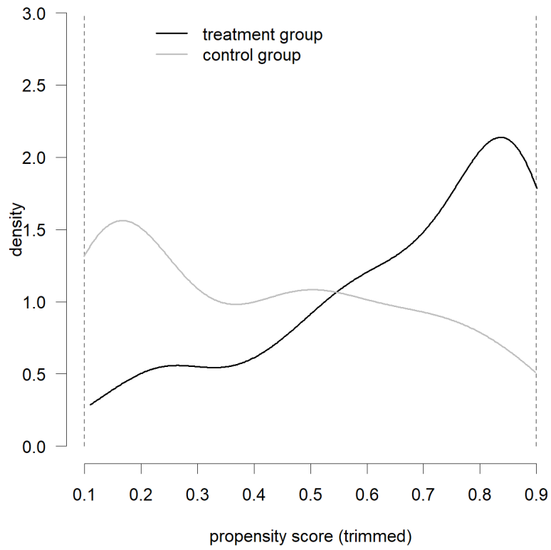
Figure 18: Density of propensity scores from Table 17
