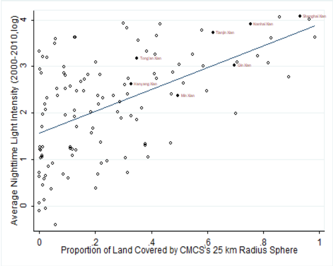
Figure 1: Correlation between CMCS Influence and Economic Development Today
