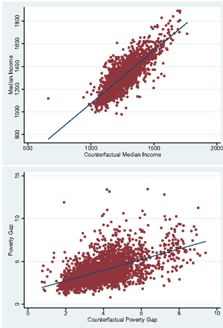
Figure B2: Instrument Strength (First Stage Regression)
