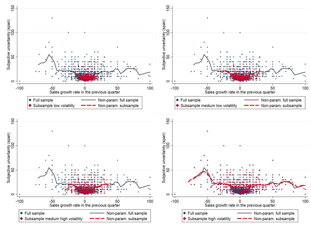
Figure 7: Relationship between subjective uncertainty (span) and sales growth in the previous quarter for four different firm volatility groups: low, medium low, medium high, and high volatility (full sample=blue, subsample=red)
