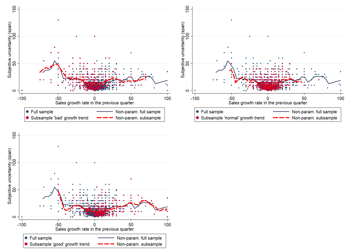
Figure 6: Relationship between subjective uncertainty (span) and sales growth in the previous quarter for three different firm trend growth groups: ‘bad’, ‘normal’, and ‘good’ trend growth (full sample=blue, subsample=red)
