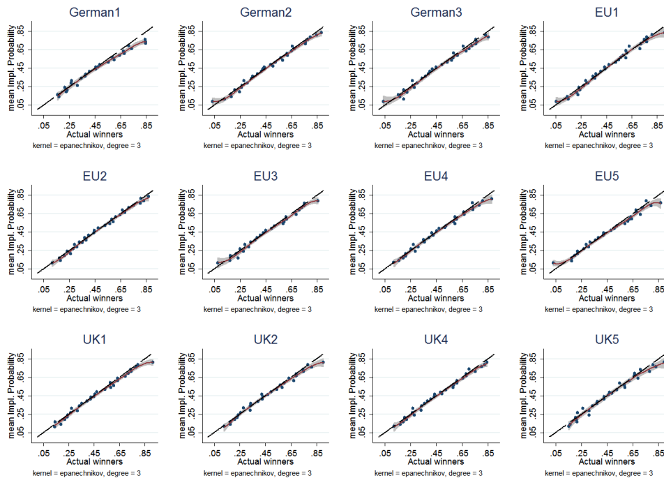
Figure 3: Implied probabilities versus outcome probabilities - Home victory
