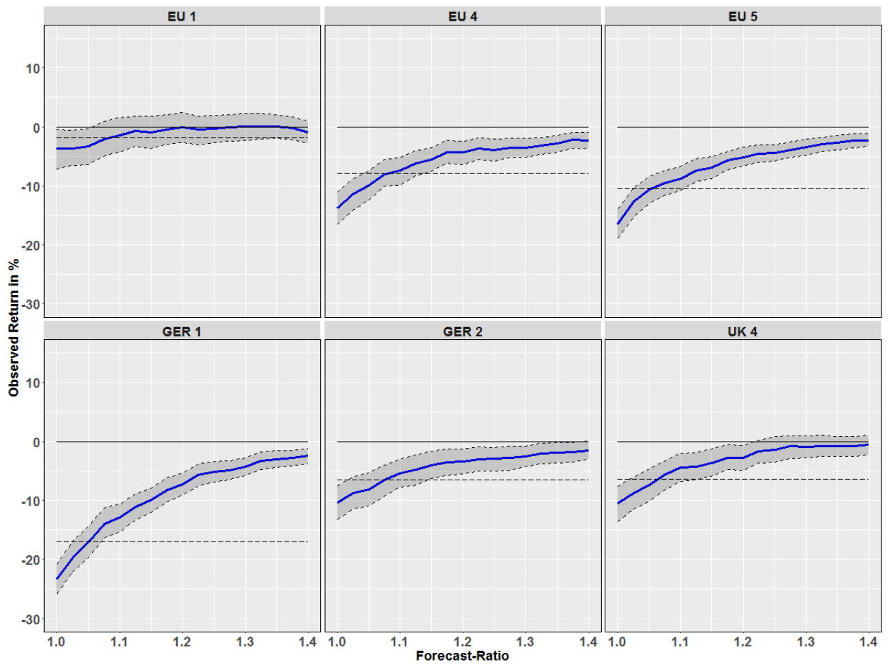
Figure 7: Observed returns conditional on different forecast-ratios
