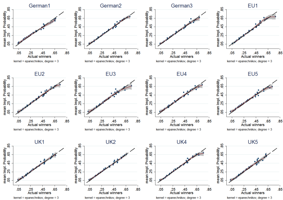
Figure 4: Implied probabilities versus outcome probabilities - Away victory
