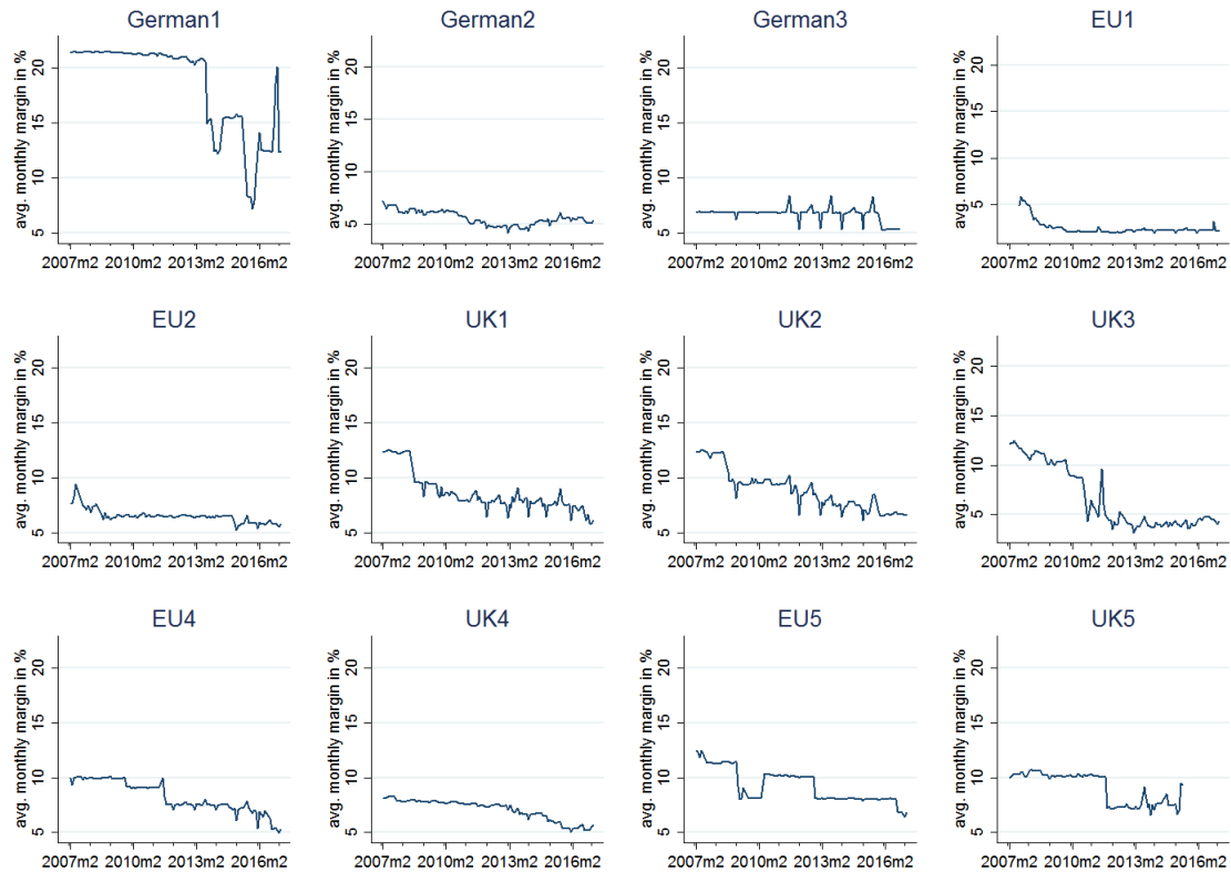
Figure 2: Evolution of bookmaker margins - German market
