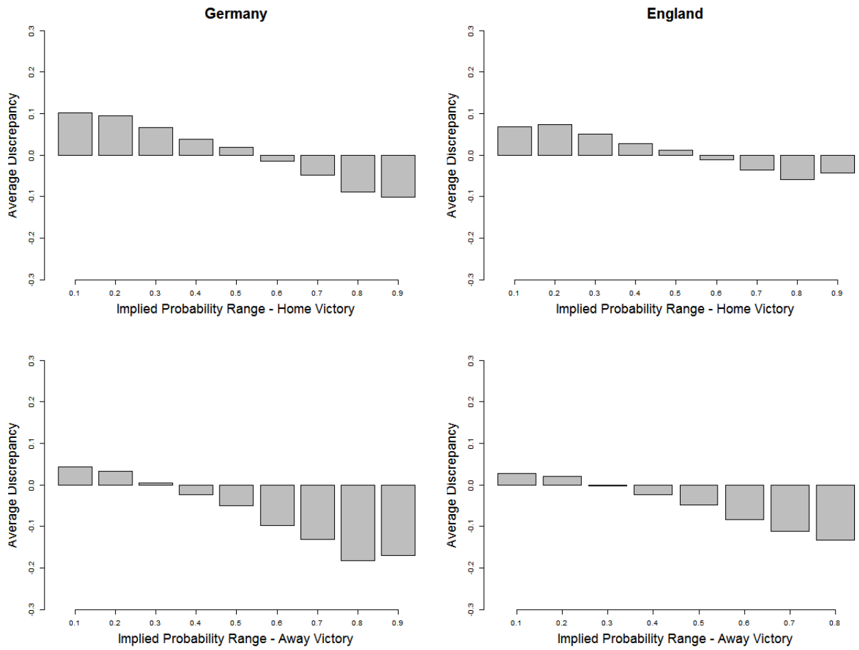
Figure 6: Discrepancy of model forecasts
