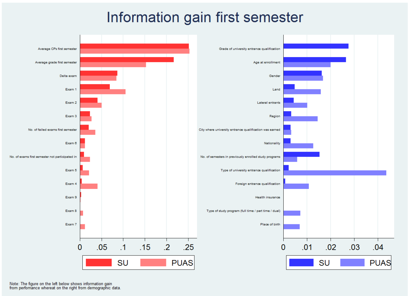
Figure 4. Bagging with random forest (information gain); First semester
