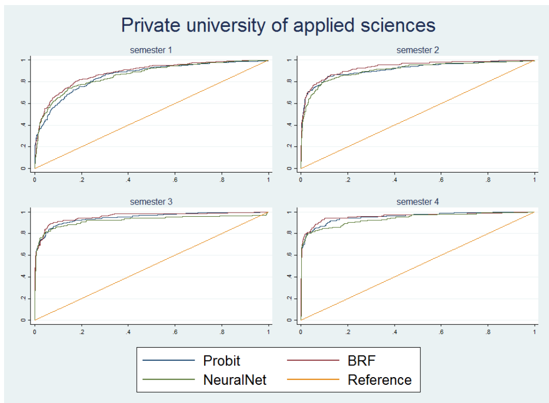
Figure 5b. ROC curve – private university of applied sciences
