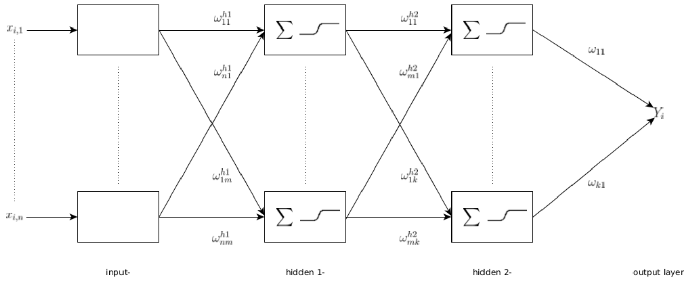
Figure 1. Neural Net
