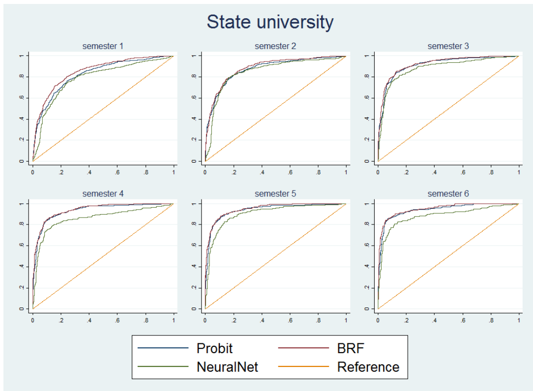
Figure 5a. ROC curve - state university
