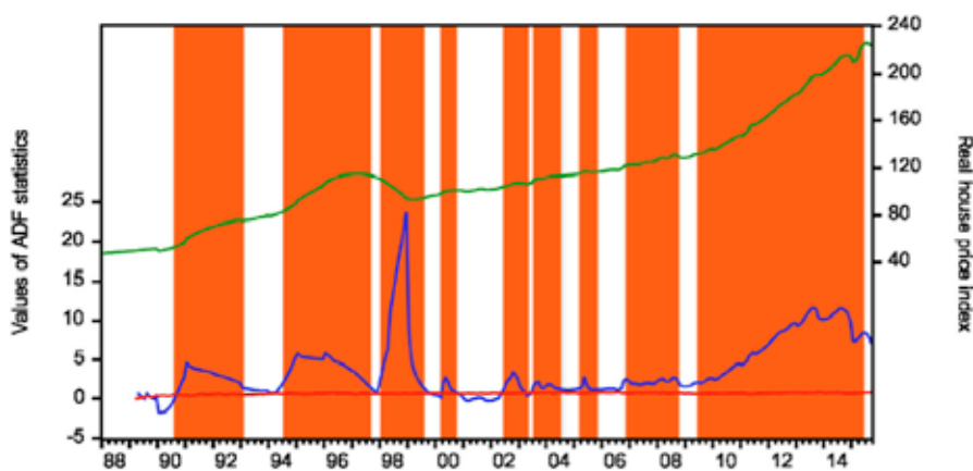
Figure 1 - Backward sup ADF sequence (BSADF) for Overall Market
