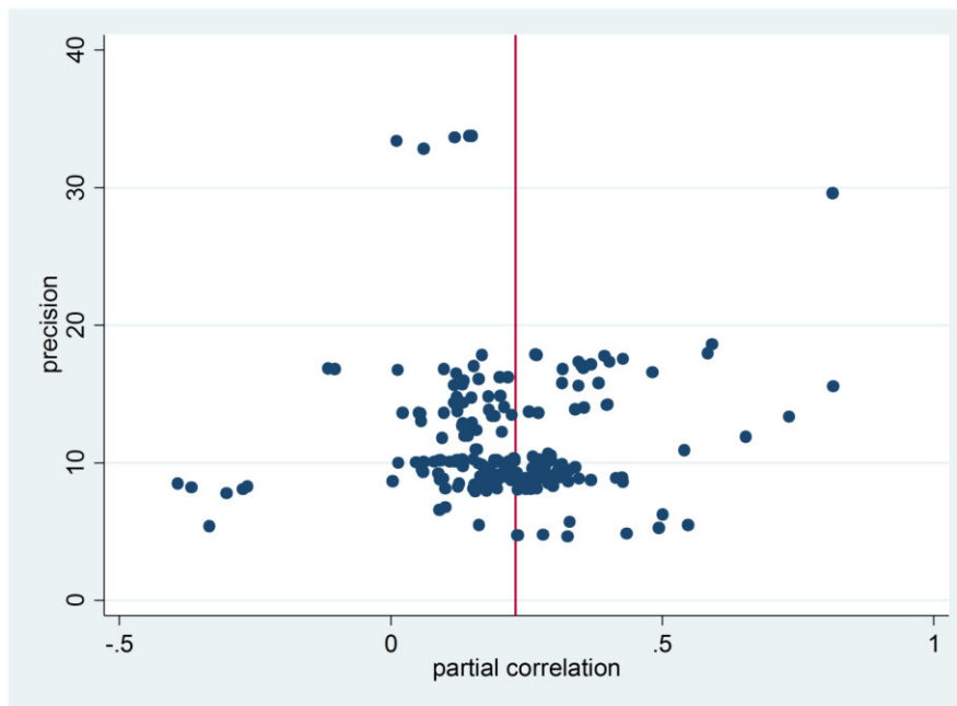
Figure 4: Funnel plot
