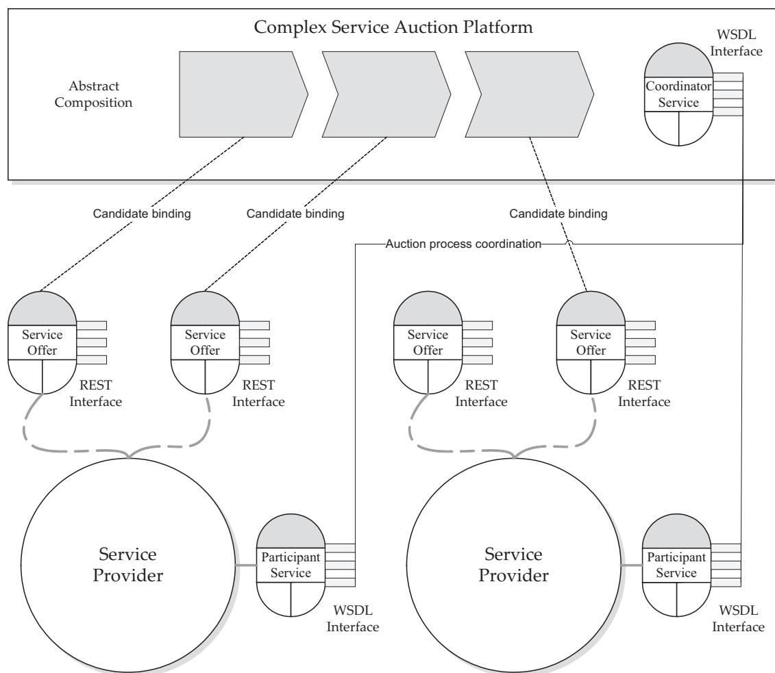
Figure 3.11 Architectural overview of the CSA.
