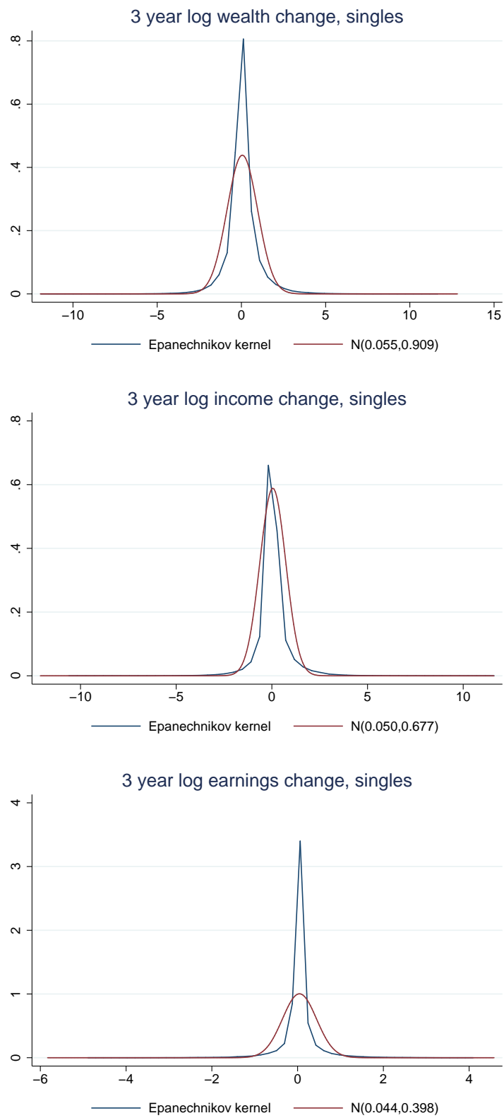
Figure 6: Wealth, income and earnings growth with corresponding normal distributions.
