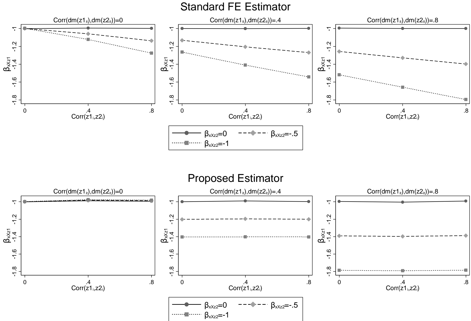
Figure 1: Standard FE Estimator vs. Proposed Estimator
