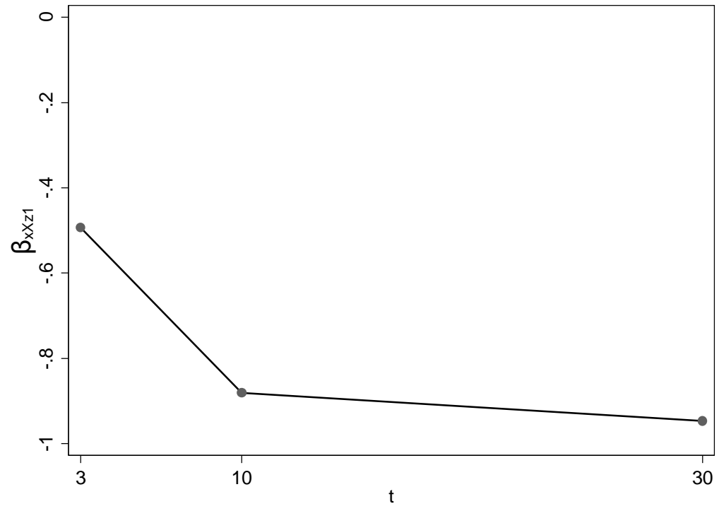
Figure 2: Effect of varying T_s on estimator without additional demeaning
