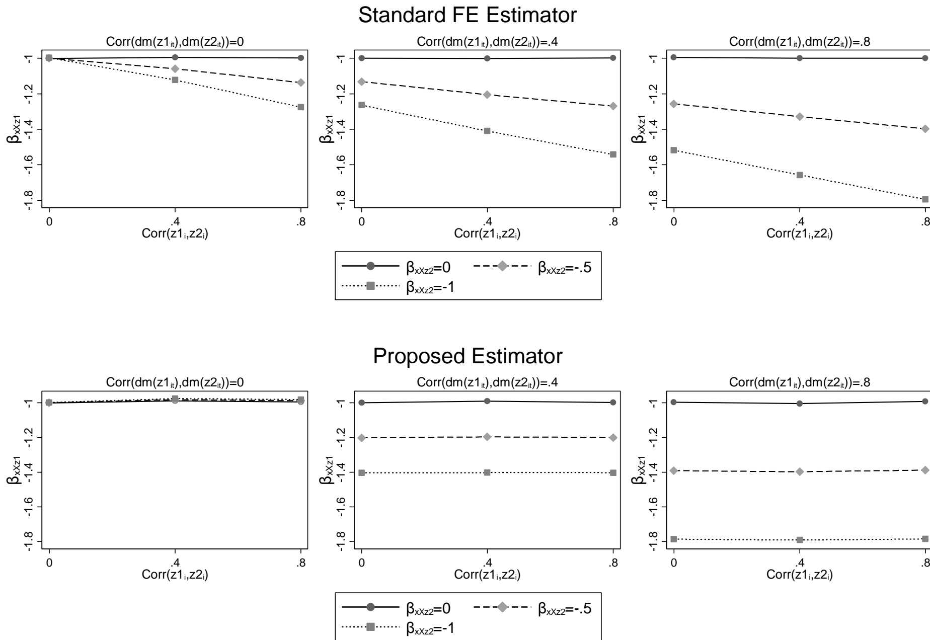
Figure 1: Standard FE Estimator vs. Proposed Estimator
