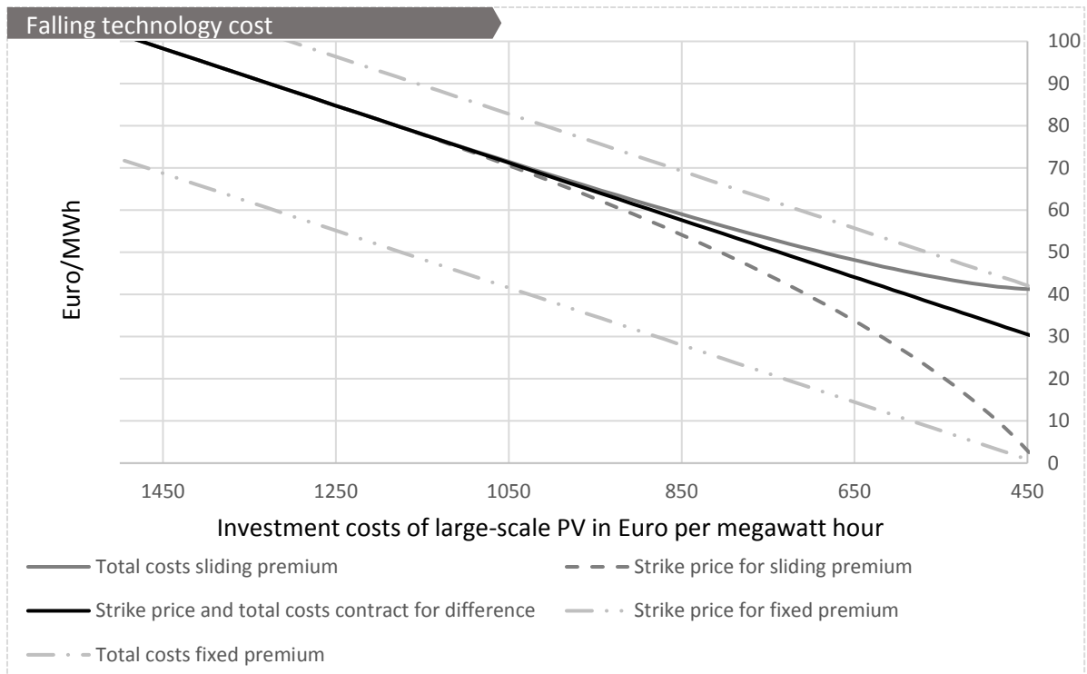
Figure 8 Evolution of Market premia and total costs to consumers of renewable energy with declining levelized costs of technology (risk free) relative to wholesale price level.
