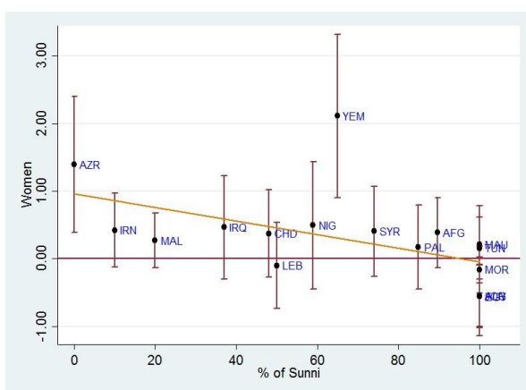
(a) Sunnis - (Corr = -0.515**)
