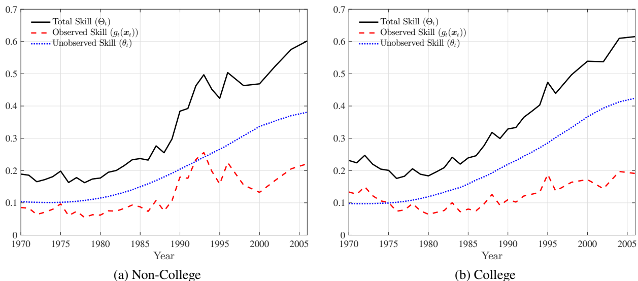
Figure 20: Skill Variances
