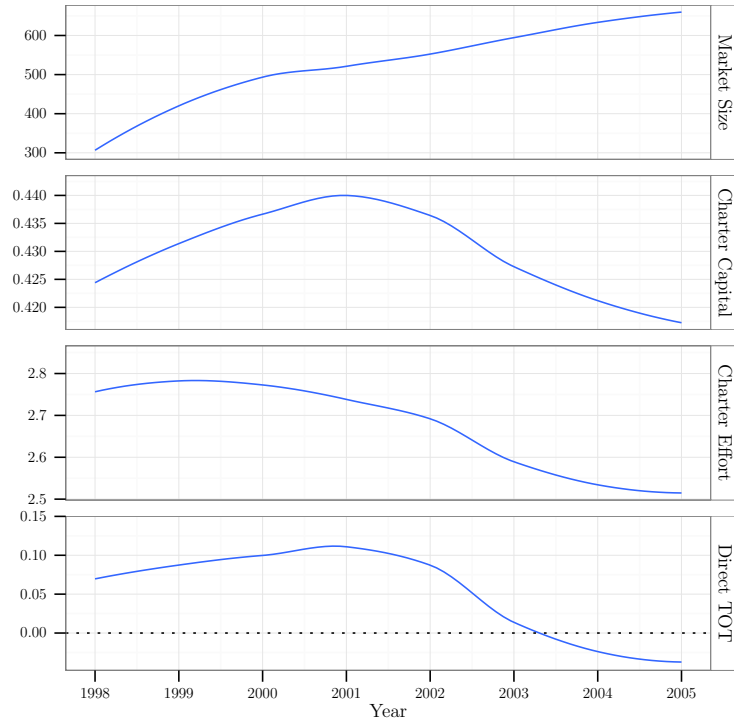
Figure 3: Model Outcomes, 1998-2005
