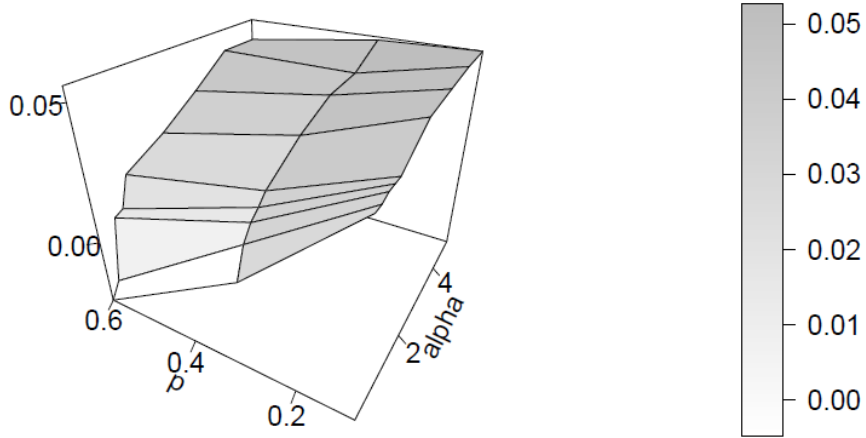
Average(|d1_MM-d2_MM|-|des1_RN-d2_RN|)
