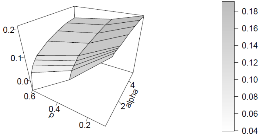
Average(|d1_MM-d2_MM|-|des1_RN-d2_RN|)
