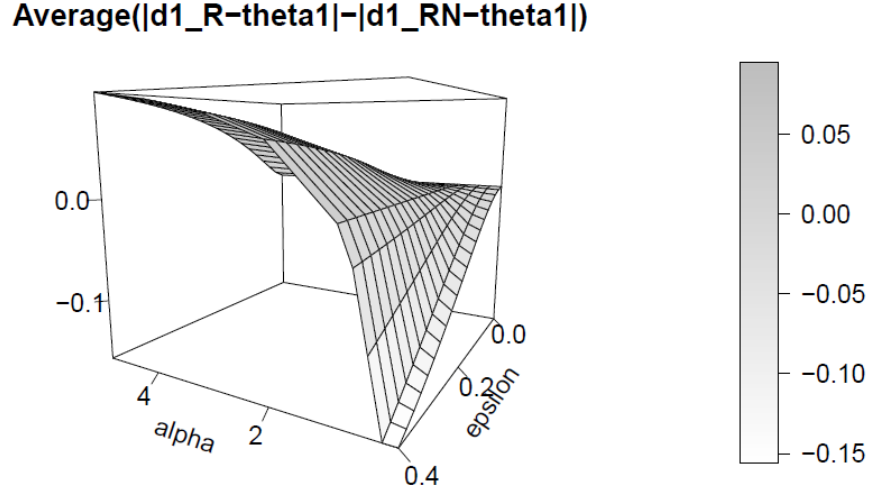
(a) Comparison of average distances between optimal risky and risk neutral level of adaptation, |d_1^R - \theta_1| - |d_1^{RN} - \theta_1| for \gamma = \frac{1}{4} , different attitudes toward risk, \alpha \in \{0.2, 0.4, 0.6, 0.8, 1, 2, 3, 4, 5\} , and different values of \epsilon \in [0, 0.4] with grid of size 0.02. Each point corresponds to the average over (\theta_1, d_2) \in [-1, 1] \times [-0.6, 0.6] with a grid of size 0.01.
