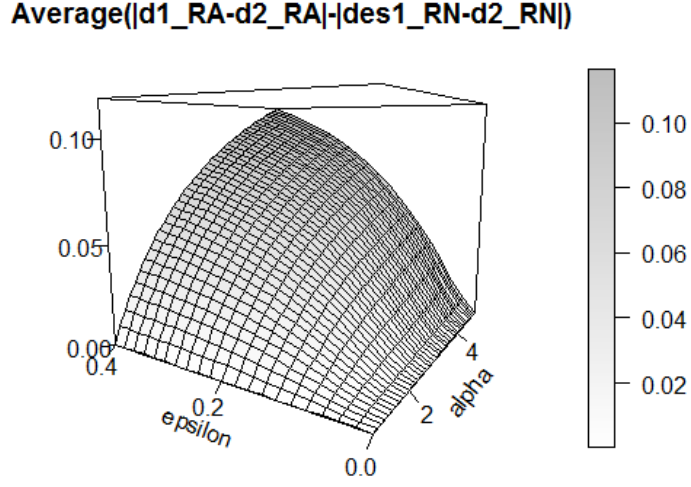
(a) Comparison of average distances between optimal risk-averse and risk-neutral decisions, |d_1^{RA} - d_2^{RA}| - |d_1^{RN} - d_2^{RN}| for \gamma = \frac{1}{4} . Each point corresponds to the average over (\nu_1, \nu_2) \in [-0.6, 0.6]^2 with a grid of size 0.05.
