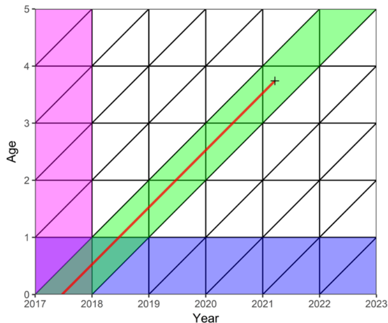
Figure 2.1: Lexis diagram
