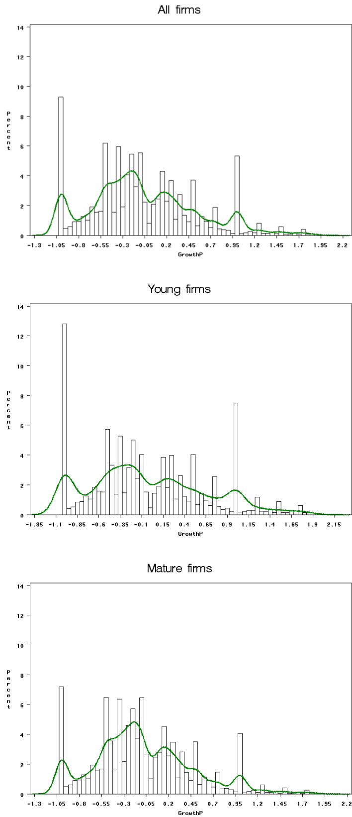
Figure 1: Kernel density of the dependent variable: g_{i,0307}
