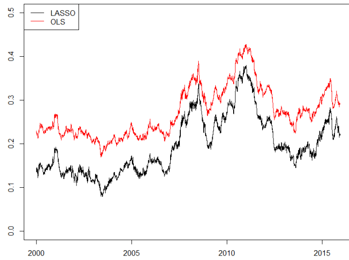
Fig. 1A. Dynamic total implied volatility spillover index for seven asset classes (the lasso method and the OLS method).
