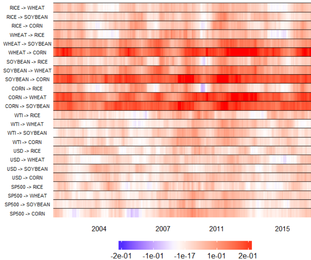
Fig. 9. Response of the food markets to shocks originating from other markets (the lasso method).
