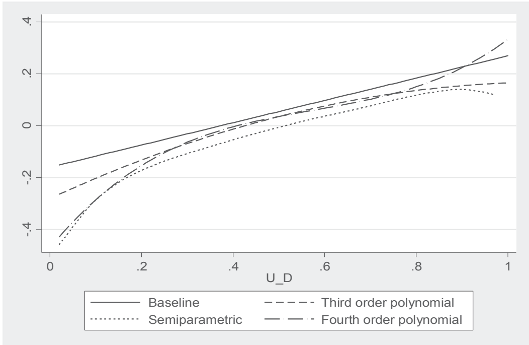
Figure 5: MTE curves - functional form robustness checks
