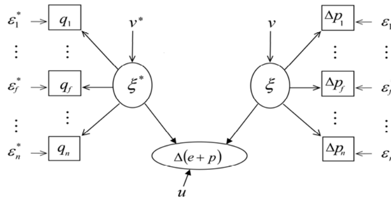
Figure 1. Static Path Diagram for Equations (4), (5) and (6)
