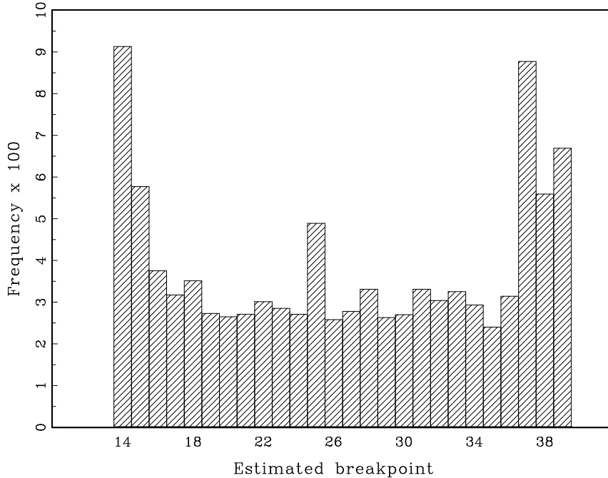
Figure 2: Distribution of \hat{t}_i^b = \arg \max(\hat{F}_{it}), T = 50 , 25% trimming at each sample end, when there is no break in the cointegrating coefficients. Pooled results from 500 Montecarlo replications for 40 units.
