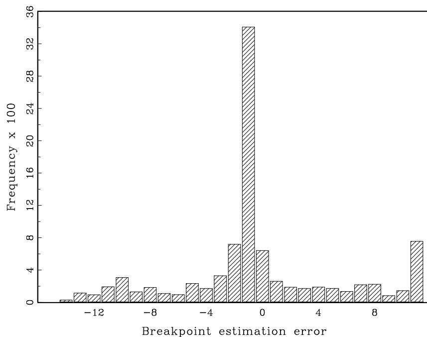
Figure 1: Distribution of the error in the estimation of the breakpoint \widehat{t}_i^b - t_i^b , where \widehat{t}_i^b = \arg \max(\widehat{F}_{it}) and t_i^b \sim \text{Uniform}[0.5T - 3, 0.5T + 3] with T = 50 . 25% trimming at each sample end, pooled results from 500 Montecarlo replications for 40 units.
