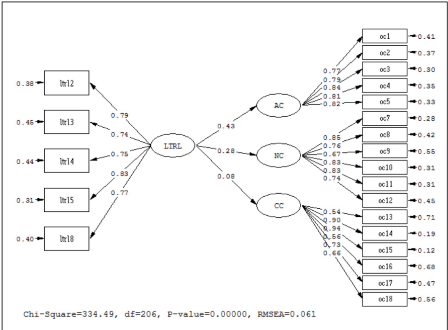
Figure 2. SEM Diagram Of The Model
