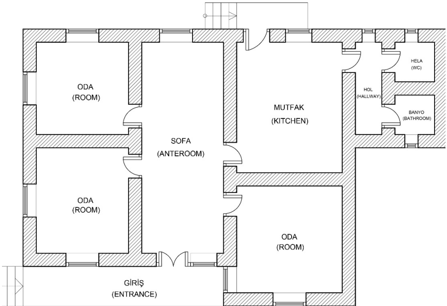
Figure 5. The Plan of Celal Gülpınar House
