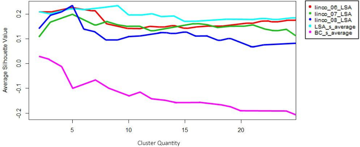
Figure 3: Average silhouette values per cluster quantity for the different cluster solutions given the LSA based distance matrix
