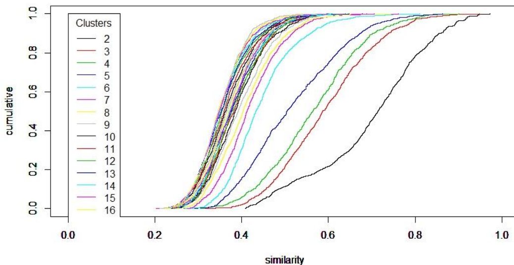
Figure 2: Stability diagram for determining the number of clusters for hybrid clustering with linear combination ( \alpha=0.6 )*
