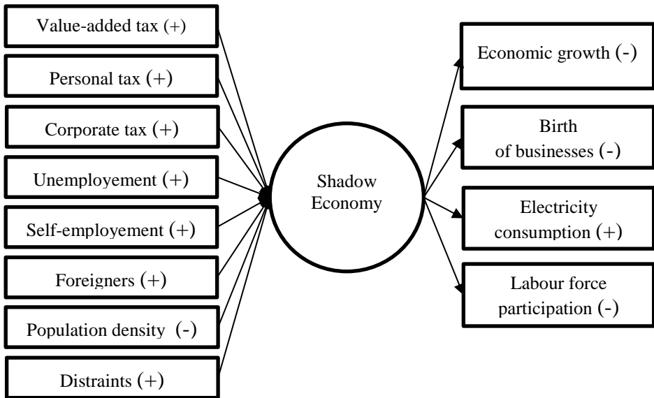
Figure 1 MIMIC model path diagram
