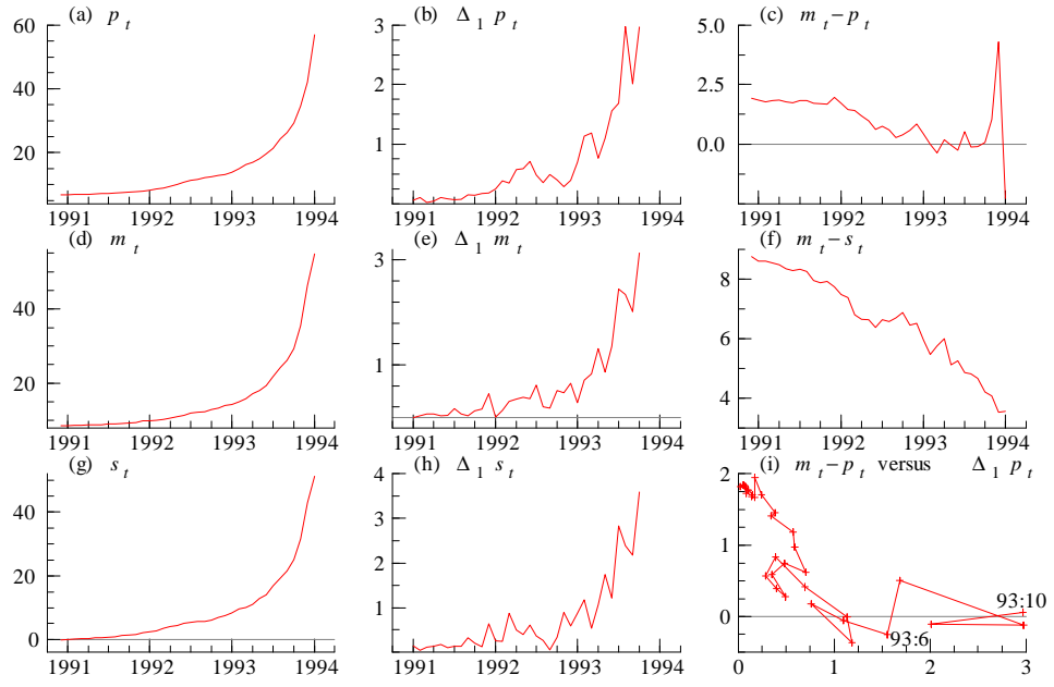
Figure 1: The series p_t, m_t, s_t and linear transformations thereof. Note that the growth rates in panels (b,e,h) are shown only until 93:10
