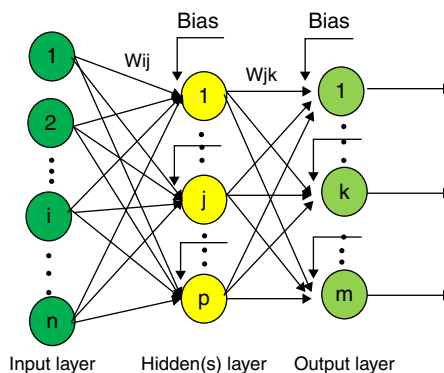
Figure 1. Multi-layer feed forward neural network structure. Elaborated by the authors.
