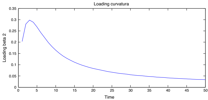
Figure 1. Behavior of the curvature factor for Colombian term structure Figure 1 shows the behavior of the curvature factor for the Colombian structure using the calculated lambda. Calculations of the authors based on proposition one.
