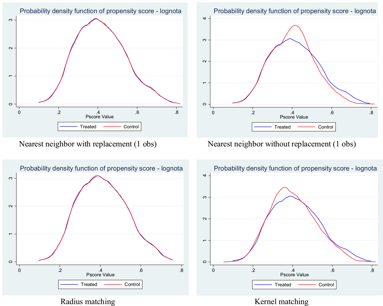
Fig. 2. Kernel density of the propensity score after pairing of 6th graders.
