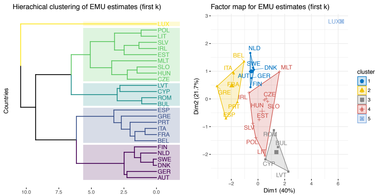
Figure A4: Alternative clustering results
