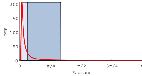
(c) J(\omega) for HP (400000)
