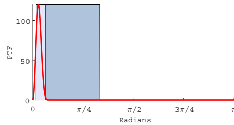
(e) J(\omega) for BK (8,30)
