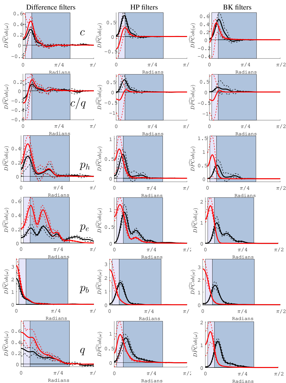
Figure 11: Dynamic power cohesion of detrended indicators across G7 countries: \Delta , HP (1600), BK (1.5,8) filter in black, \Delta_4 , HP (400000), and BK (8,30) filter in red
