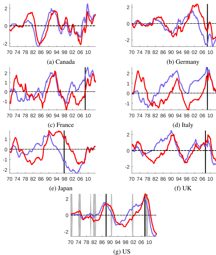
Figure 19: Credit-to-GDP gap: Two-sided (red) versus one-sided (purple) HP filter
