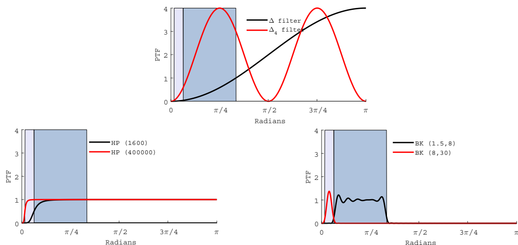
Figure 3: (Trend) stationary time series: power transfer functions, H(\omega)
