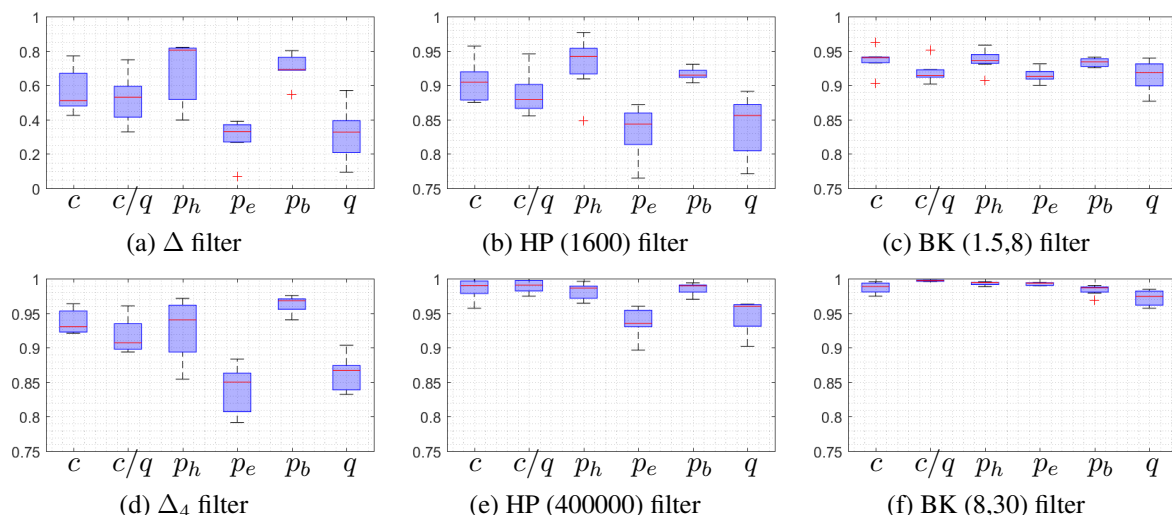
Figure 8: First-order autocorrelation of detrended indicators across G7 countries
