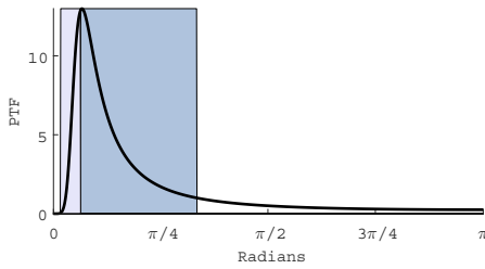
(b) J(\omega) for HP (1600)
