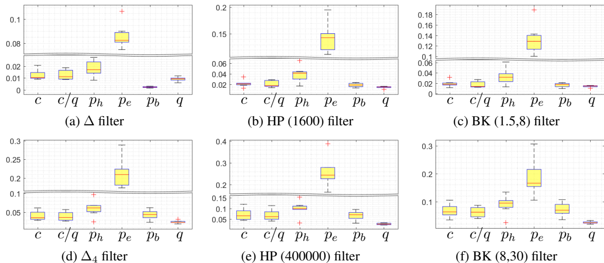
Figure 7: Standard deviation of detrended indicators across G7 countries
