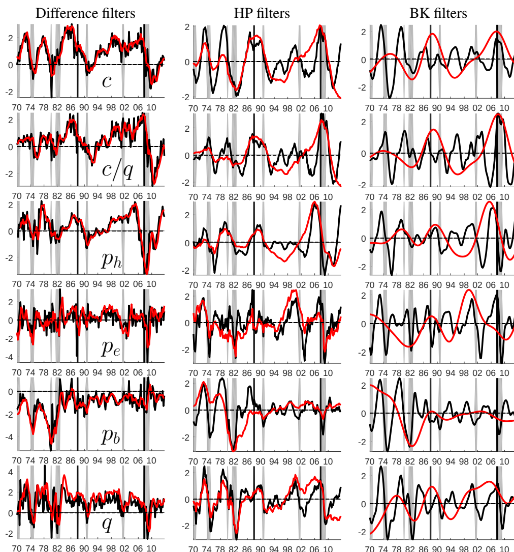
Figure 6: Detrended US' financial and business cycle indicators: \Delta , HP (1600), BK (1.5,8) filter in black, \Delta_4 , HP (400000), and BK (8,30) filter in red
