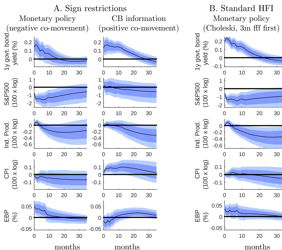
Figure B.3: Impulse responses of y_t to monetary policy and central bank information shocks, model with Industrial Production and Consumer Price Index. Median (line), percentiles 16-84 (darker band), percentiles 5-95 (lighter band).
