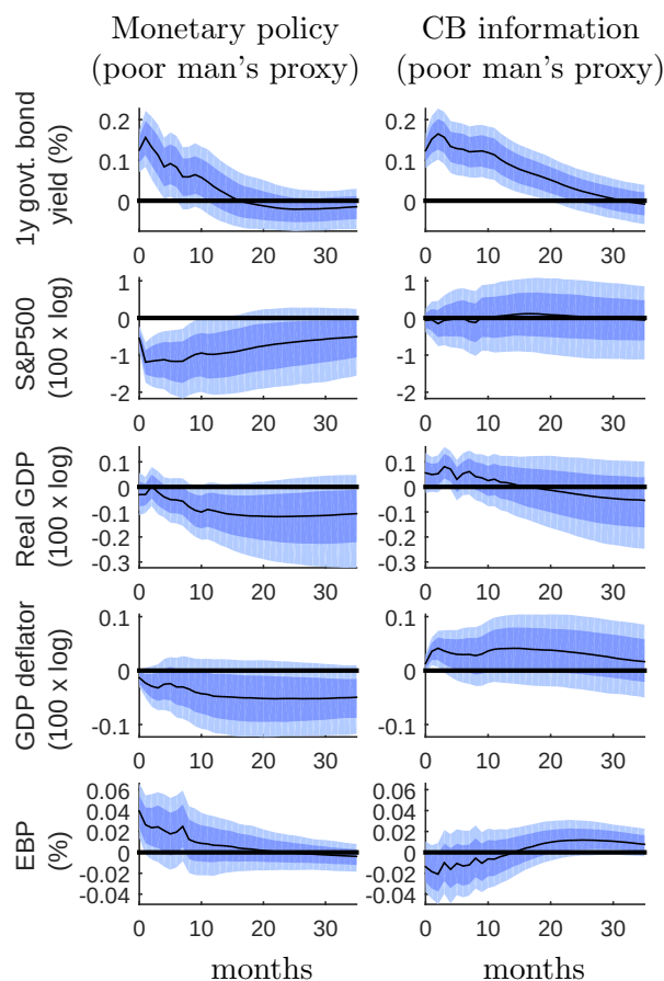
Figure 3: Impulse responses to one standard deviation shocks, baseline VAR with ‘poor man’s’ sign restrictions. Median (line), percentiles 16-84 (darker band), percentiles 5-95 (lighter band).
