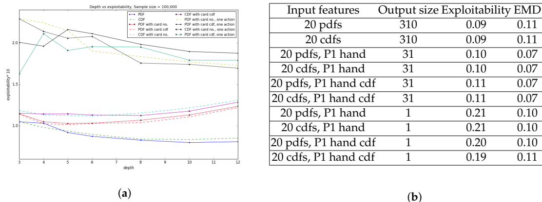
Figure 6. Exploitability vs. decision-tree depth (Figure 6a). Performance for depth-5 tree (Figure 6b).
