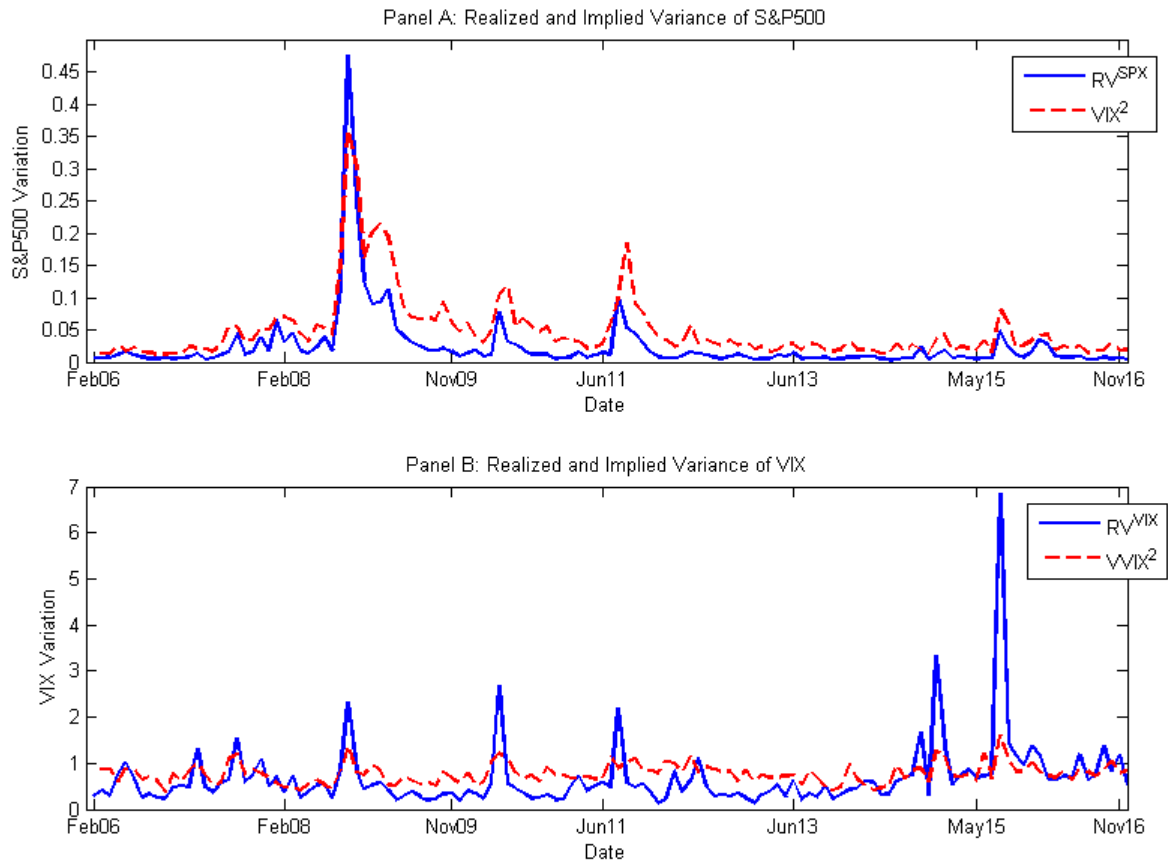
Figure 2: Realized and Implied Variance Measures
