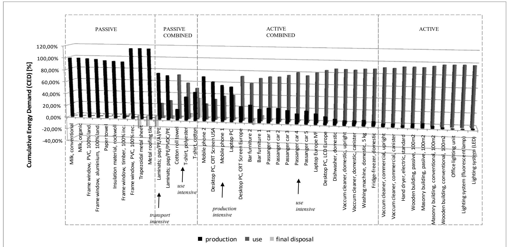
Figure 2. Environmental impact (as CED) of various life cycle stages for the 47 analysed products
