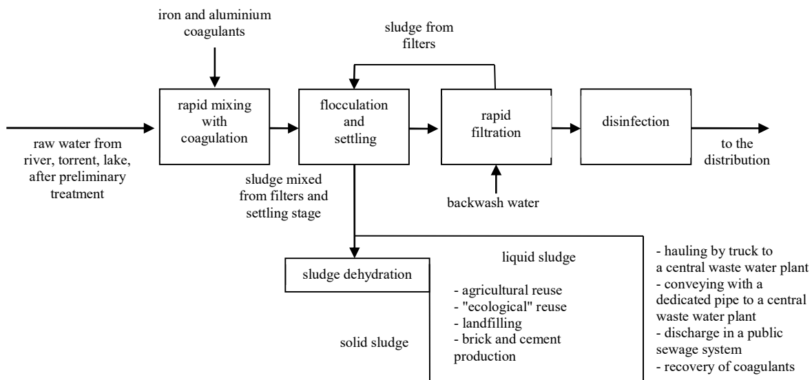
Figure 1. Production and disposal of solid and liquid sludge in a Water Treatment Plant
