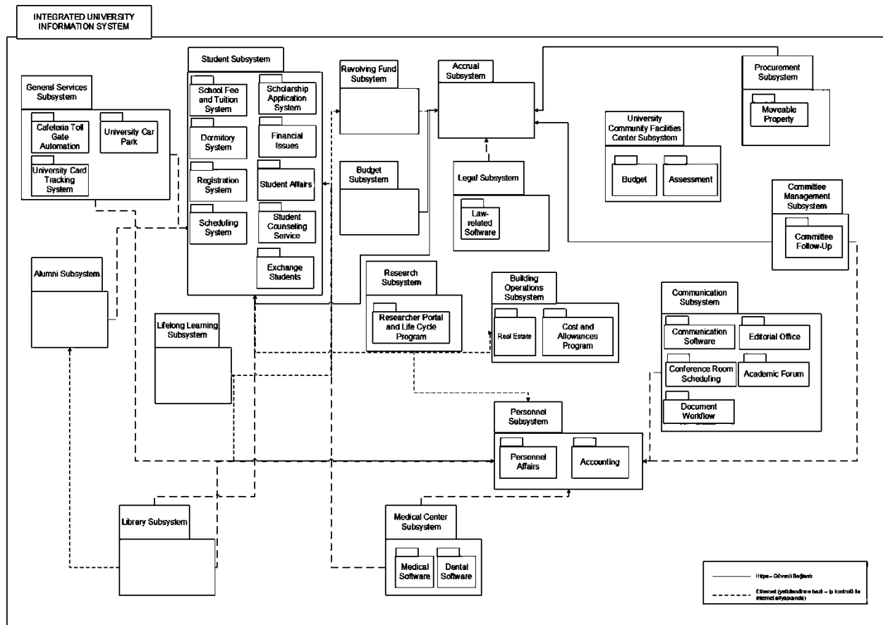
Figure 2: Package Diagram for the University Administration System
