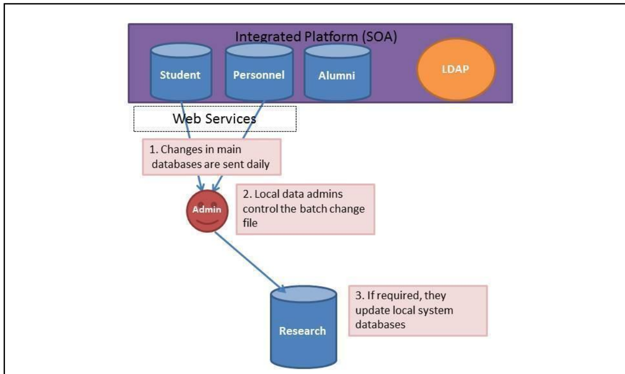
Figure 5: Local Database Update Workflow based on Web Services for IUIS
