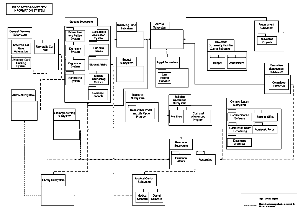
Figure 2: Package Diagram for the University Administration System
