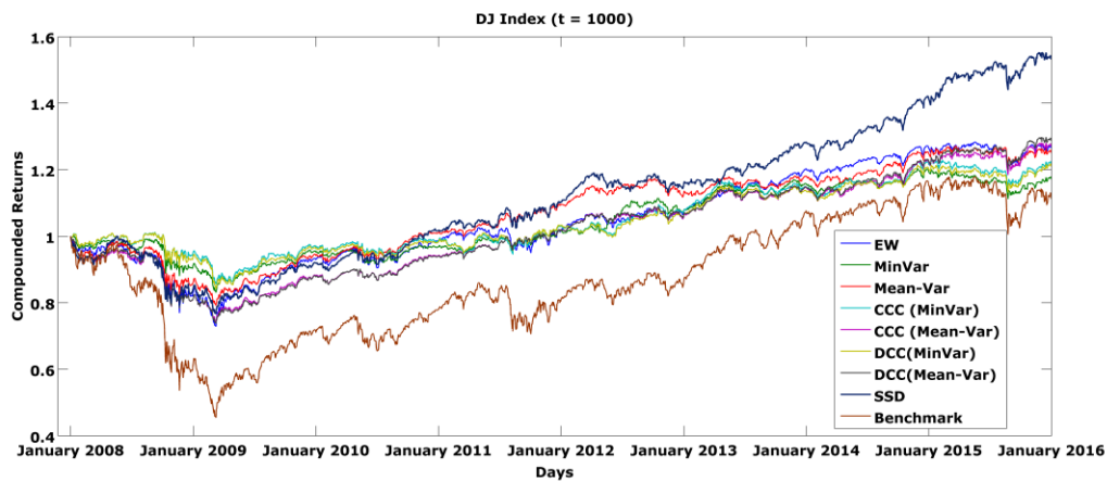
Figure 2. Compounded (on daily basis) returns of portfolios consisting of DJ stocks, t = 1000 .
