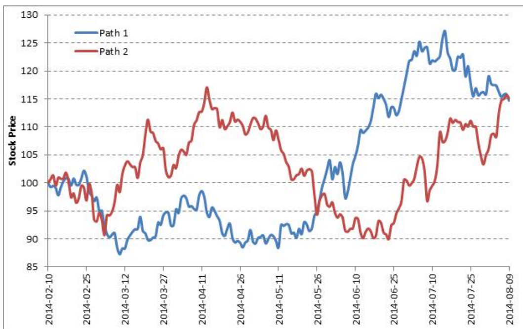
Figure 3. Two simulated price paths of some stock with a 30% volatility over a six month period
