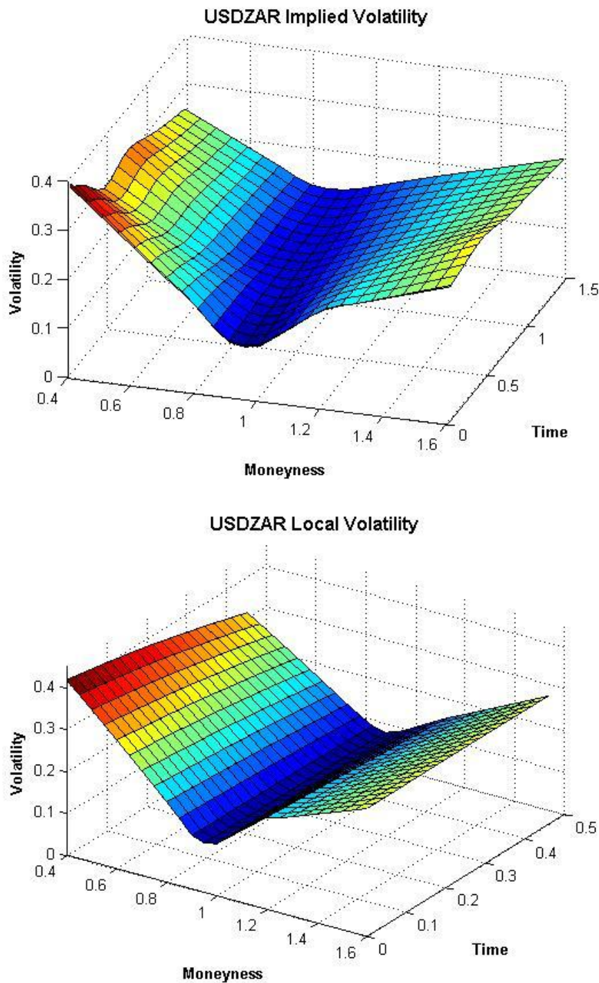
Figure 9. USDZAR implied and local volatility surfaces on 28 May 2014.
