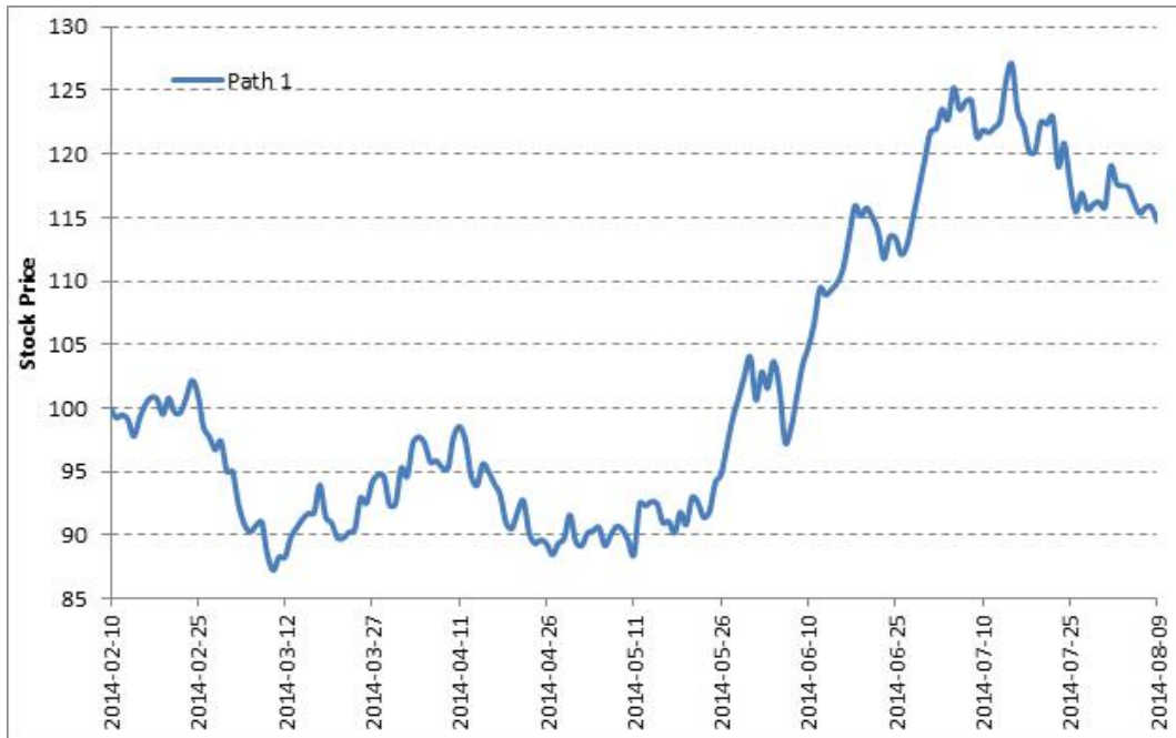
Figure 2. One simulated price path of some stock with a 30% volatility over a six month period
