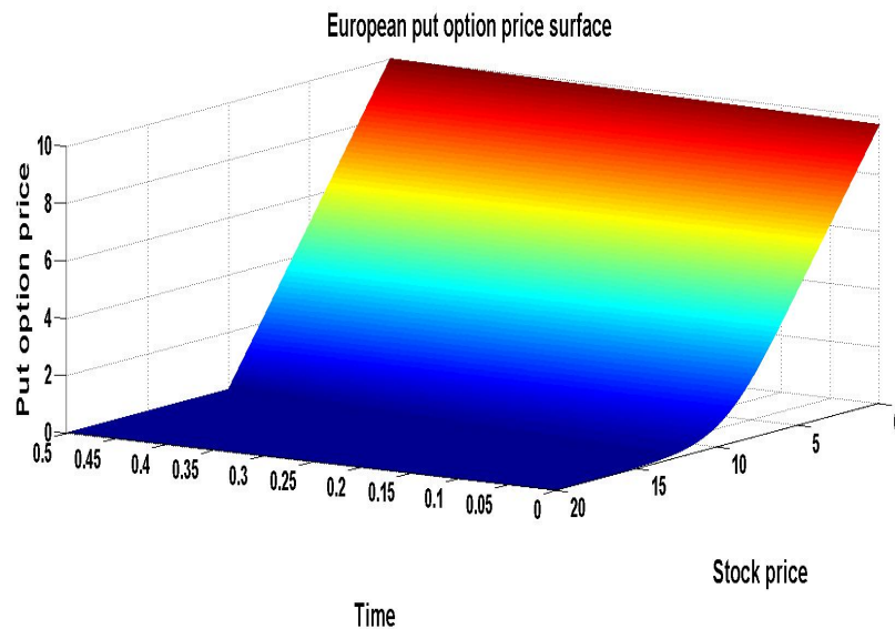
Figure 7. Collateralized European put option surface using the PDE approach with parameters: S_0 \in [0, 20] , K = 10 , dt = 0.0001 (5000 time increments), ds = 0.02 (1000 space increments), T = 0.5 , t \in [0, T] , r_C = 0.04 , r_R = 0.05 , r_F = 0.06 , r_D = 0.01 , \sigma = 0.3 and \theta = 1 .
