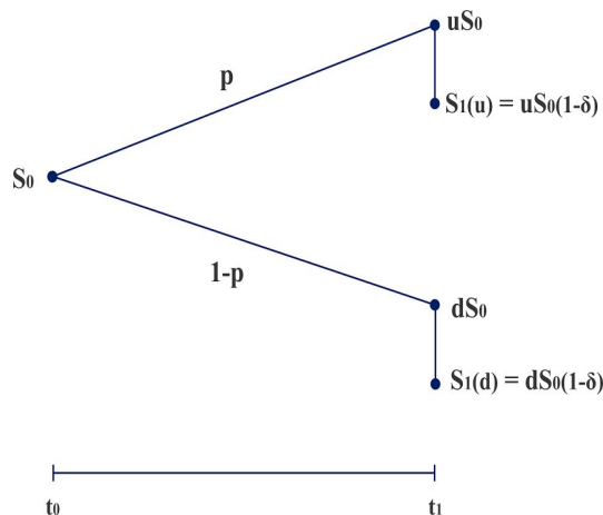
Figure 2. One-period binomial asset pricing model with a discrete dividend.
