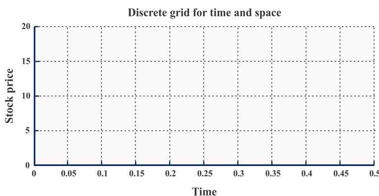
Figure 6. Discrete grid of time and space.
