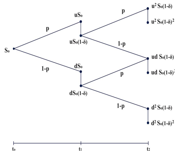
Figure 3. Two-period binomial asset pricing model with discrete dividends.
