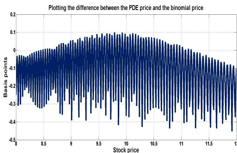
Figure 9. Difference between the PDE price and the binomial lattice price for a collateralized European put option with parameters: S_0 \in [8, 12] , K = 10 , dt = 0.0001 (5000 time increments), ds = 0.02 (1000 space increments), T = 0.5 , r_C = 0.04 , r_R = 0.05 , r_F = 0.06 , r_D = 0.01 , \sigma = 0.3 and \theta = 1 .
