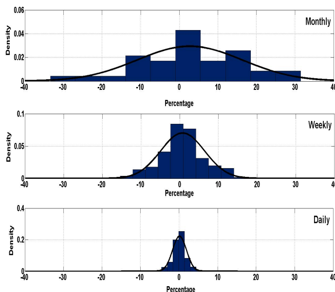
Figure 11. The distribution of the default risk of a collateralized European put option for three different recollateralization periods with parameters: S_0 = 10 , K = 10 , r_C = 0.04 , r_R = 0.05 , r_F = 0.06 , r_D = 0.01 , T = 3 and \sigma = 0.3 .
