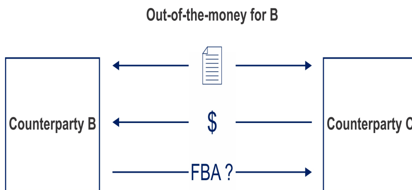
Figure 4. Illustrating a trade graphically between Counterparties B and C when Counterparty B is out-of-the-money.
