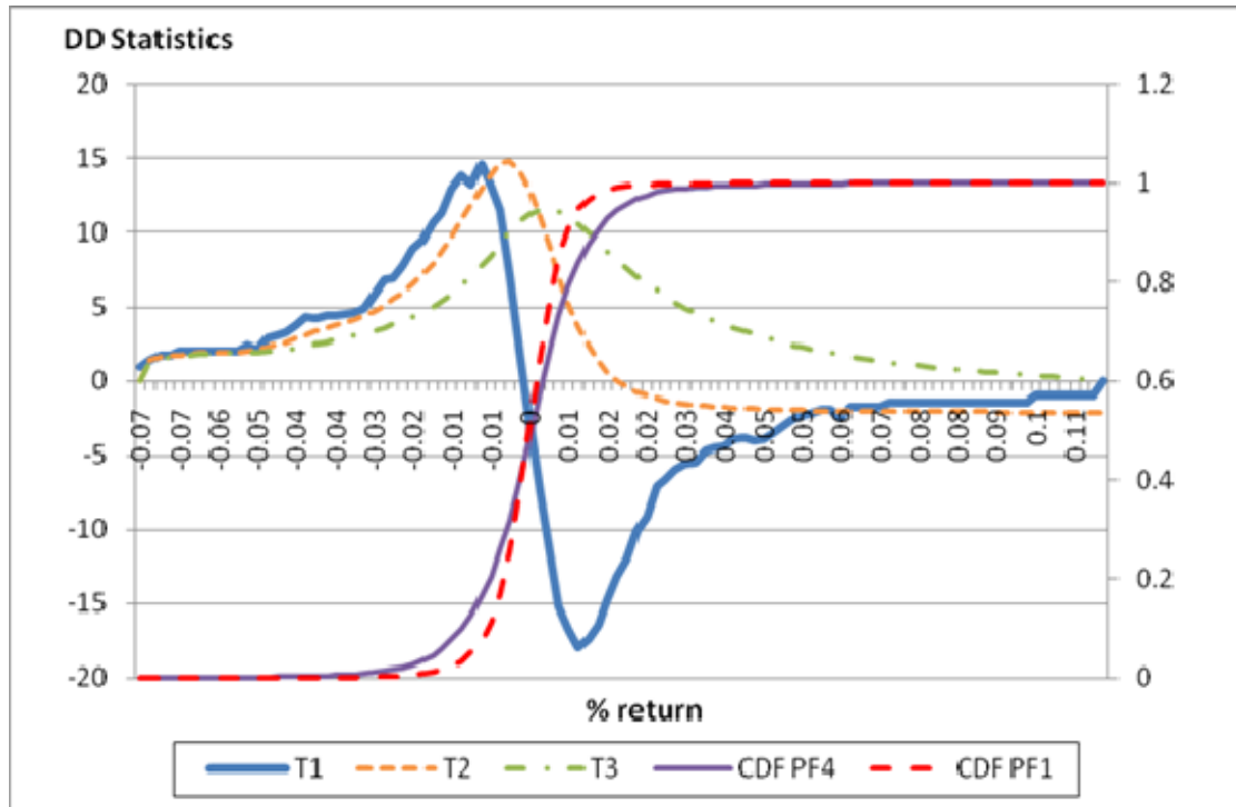
Figure 3. Plot of the CDF of the daily returns of the third domestic diversified portfolio (DOD3) and the 13 international diversified portfolios (IND13) and their DD statistics.
