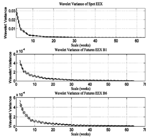
Figure 1: Estimated wavelet variance of spot and futures returns
