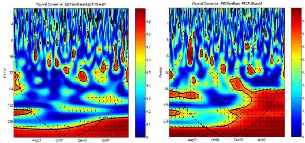
Figure 3: Cross-wavelet coherency and phase plots between spot base and futures base
