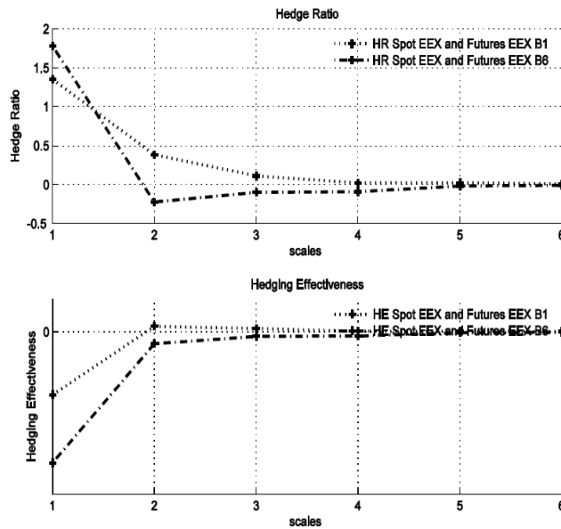
Figure 4: Hedge ratio and hedging effectiveness with different wavelet domains
