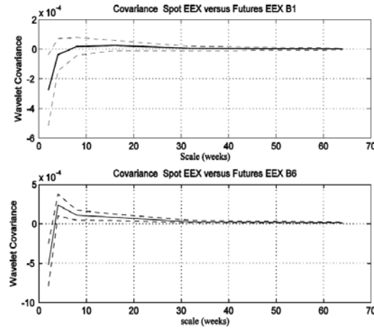
Figure 2: Estimated wavelet covariance between the spot and futures returns
