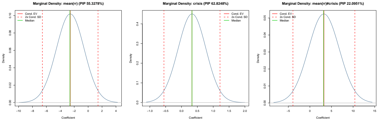
Figure 5: GDP growth, posterior marginal densities of selected coefficients
