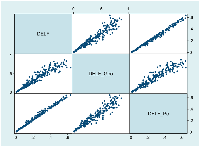
Figure C.8: Scatter plots of the differently weighted DELFL values
