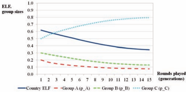
Figure 1.2: Results of dynamic modeling per round
