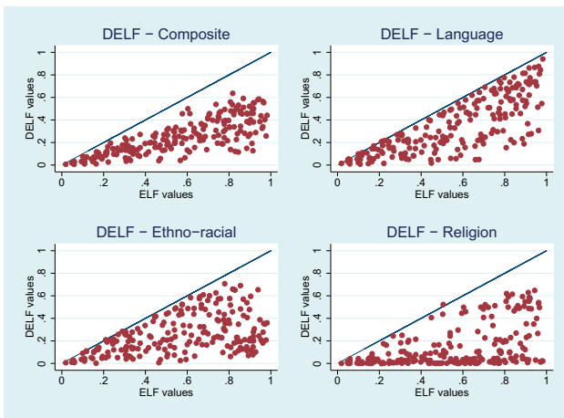
Figure 3.2: Combined and single characteristic DEL F values against ELF values.
