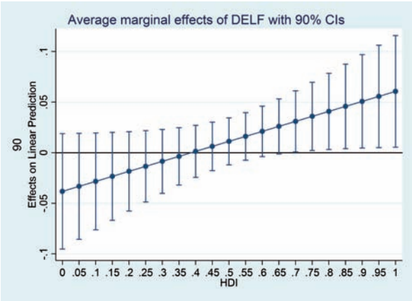
(b) Regression (5)
