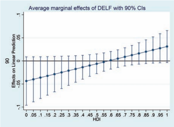
(a) Regression (4)
