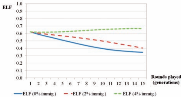
Figure 1.6: Overall country ELF values for different immigration rates
