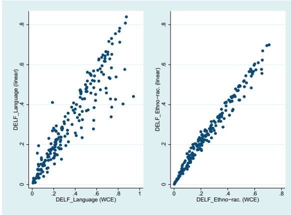
Figure C.4: DELF values based on WCE similarity values against linear scale DELF values per characteristic
