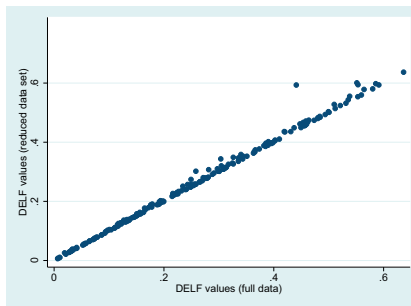
Figure C.2: Original DELf values against reduced data set
