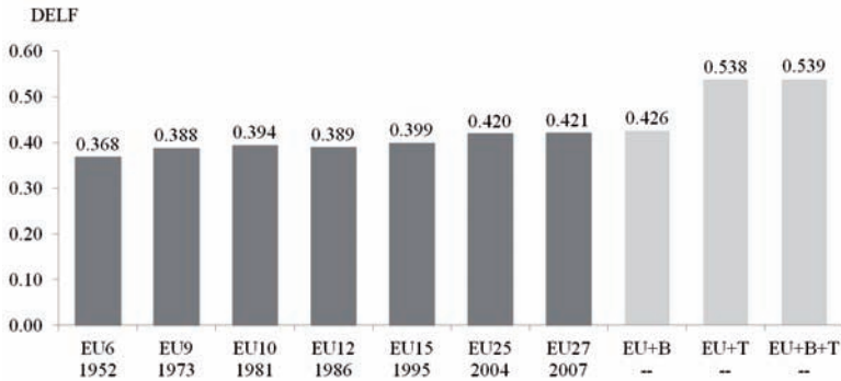
Figure 3.3: Average DEL F values of the EU per enlargement wave
