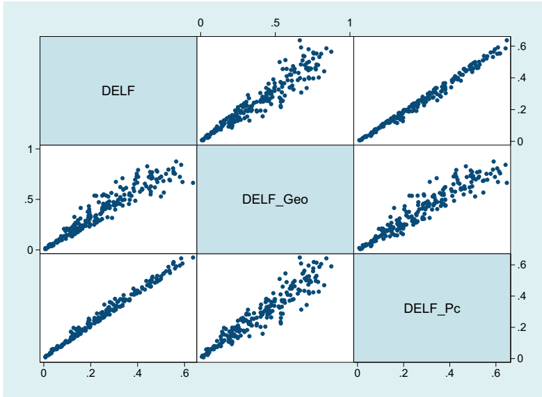
Figure C.8: Scatter plots of the differently weighted DELF values
