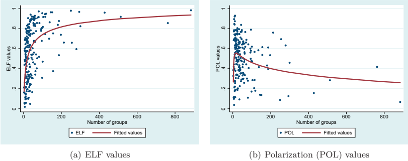
Figure C.6: ELF and POL values against number of groups for 210 countries based on WCE data
