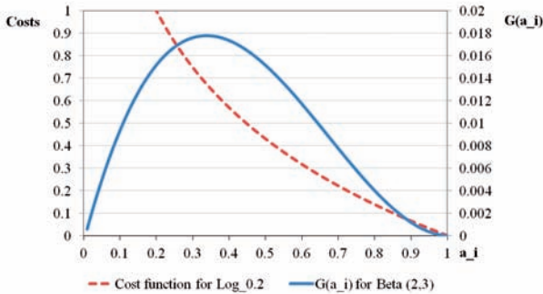
Figure 1.1: Density function for selected B(2,3) distribution and cost function with \theta = 0.2
