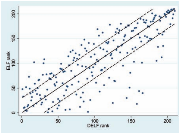
Figure 4.1: Scatter plot of ELF and DELf rank values
