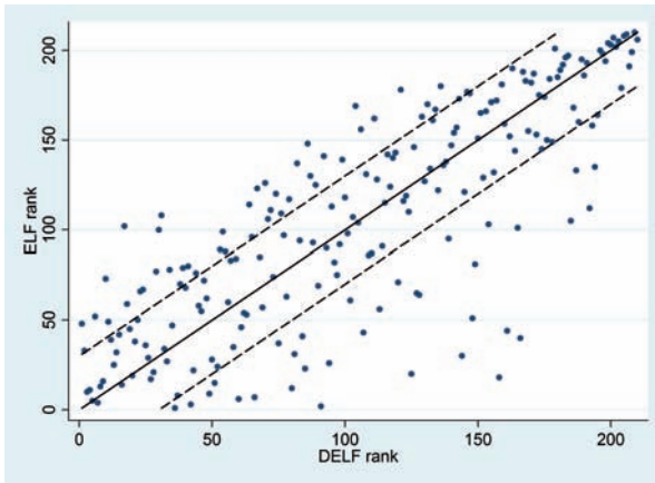
Figure 4.1: Scatter plot of ELF and DELFL rank values
