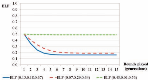
Figure 1.3: ELF values for different group constellations
