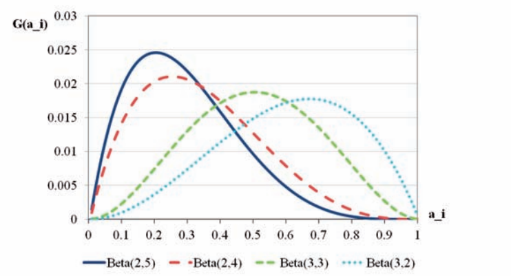
Figure A.2: Density functions for selected B(\alpha,\beta) distributions
