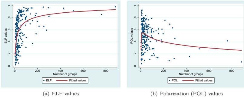
Figure C.6: ELF and POL values against number of groups for 210 countries based on WCE data
