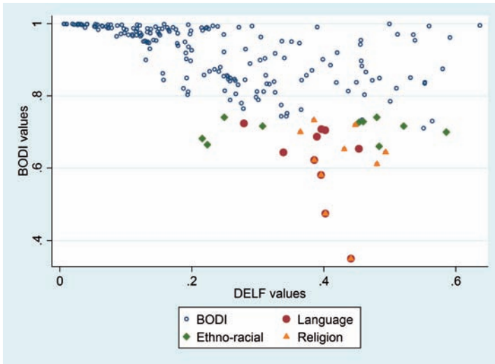
Figure C.9: Scatter plots of BODI and DELf values. For countries with highest deviations, responsible characteristics marked
