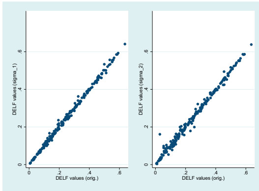
Figure C.1: Original DELf values against newly created random data sets
