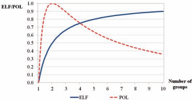
Figure 3.1: ELF and POL values depending on the number of equally sized groups
