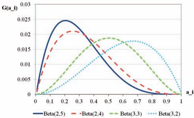
Figure A.2: Density functions for selected B(\alpha, \beta) distributions
