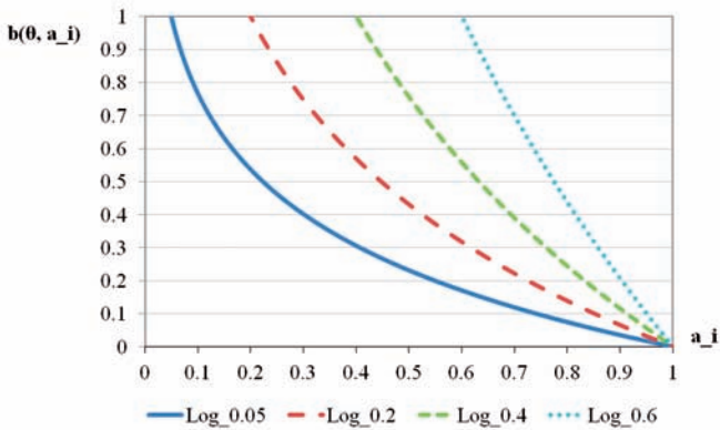
Figure A.3: Cost functions for selected levels of \theta
