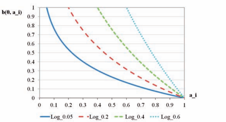
Figure A.3: Cost functions for selected levels of \theta
