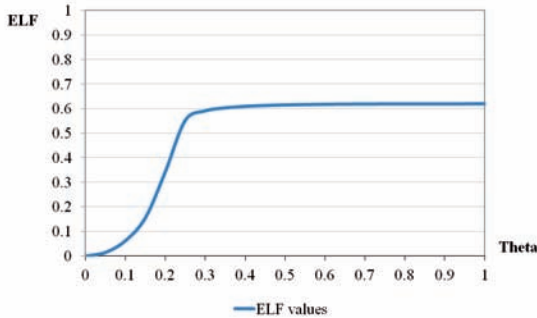
Figure 1.4: ELF values after 15 rounds depending on \theta values
