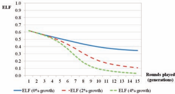
Figure 1.5: ELF values for different growth rates
