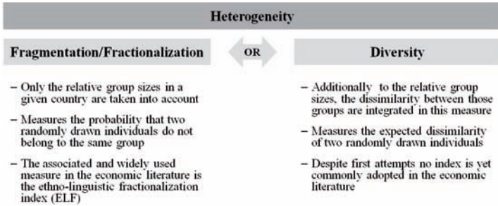
Figure 0.1: Difference of fragmentation and diversity measure
