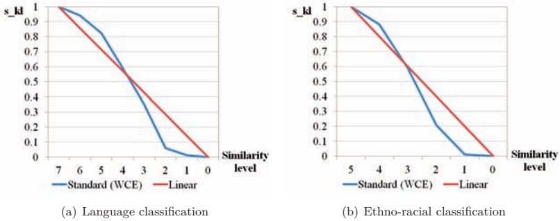
Figure C.3: Used similarity values \bar{s}_{kl} vs. linear similarity levels
