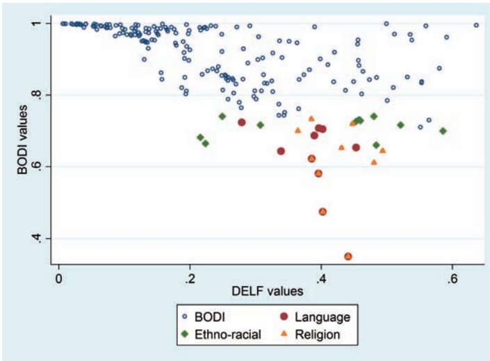
Figure C.9: Scatter plots of BODI and DELFL values. For countries with highest deviations, responsible characteristics marked
