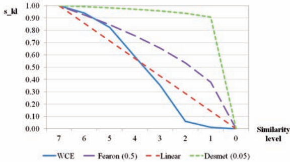
Figure C.5: Similarity functions depending on different concavity assumptions
