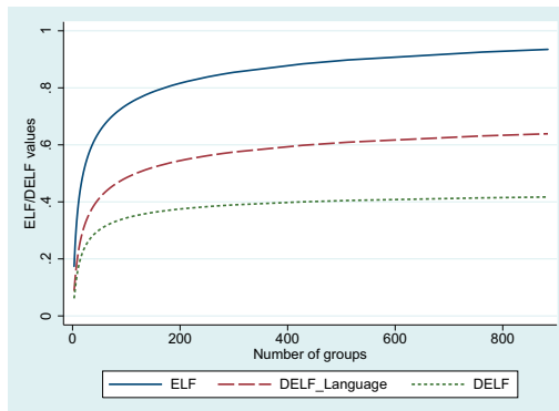
Figure C.7: Fitted ELF and DEL F values against number of groups for all 210 countries
