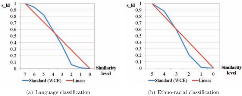
Figure C.3: Used similarity values \bar{s}_{kl} vs. linear similarity levels
